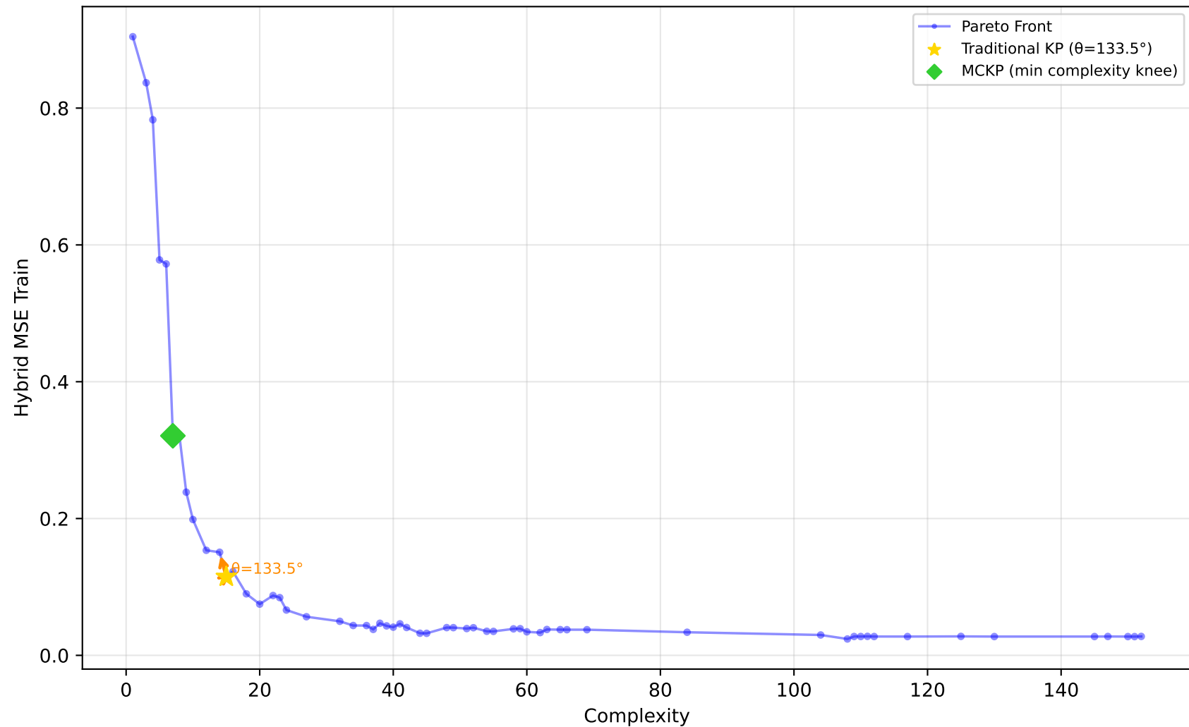
227_cpu_small - Run 14 - SVP - Hybrid MSE Train \lambda_1=0.00, \lambda_2=1.00, \lambda_3=0.00 | Difficulty: 1.00 | Method: hmr
