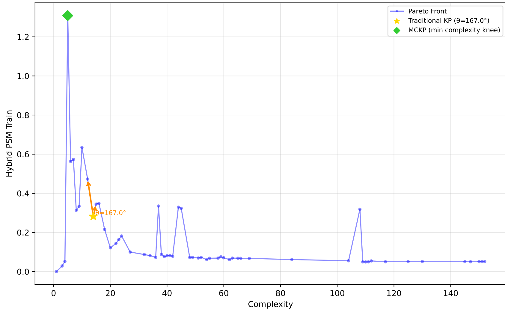
227_cpu_small - Run 14 - SVP - Hybrid PSM Train \lambda_1=0.00, \lambda_2=0.80, \lambda_3=0.30 | Difficulty: 1.00 | Method: hmr
