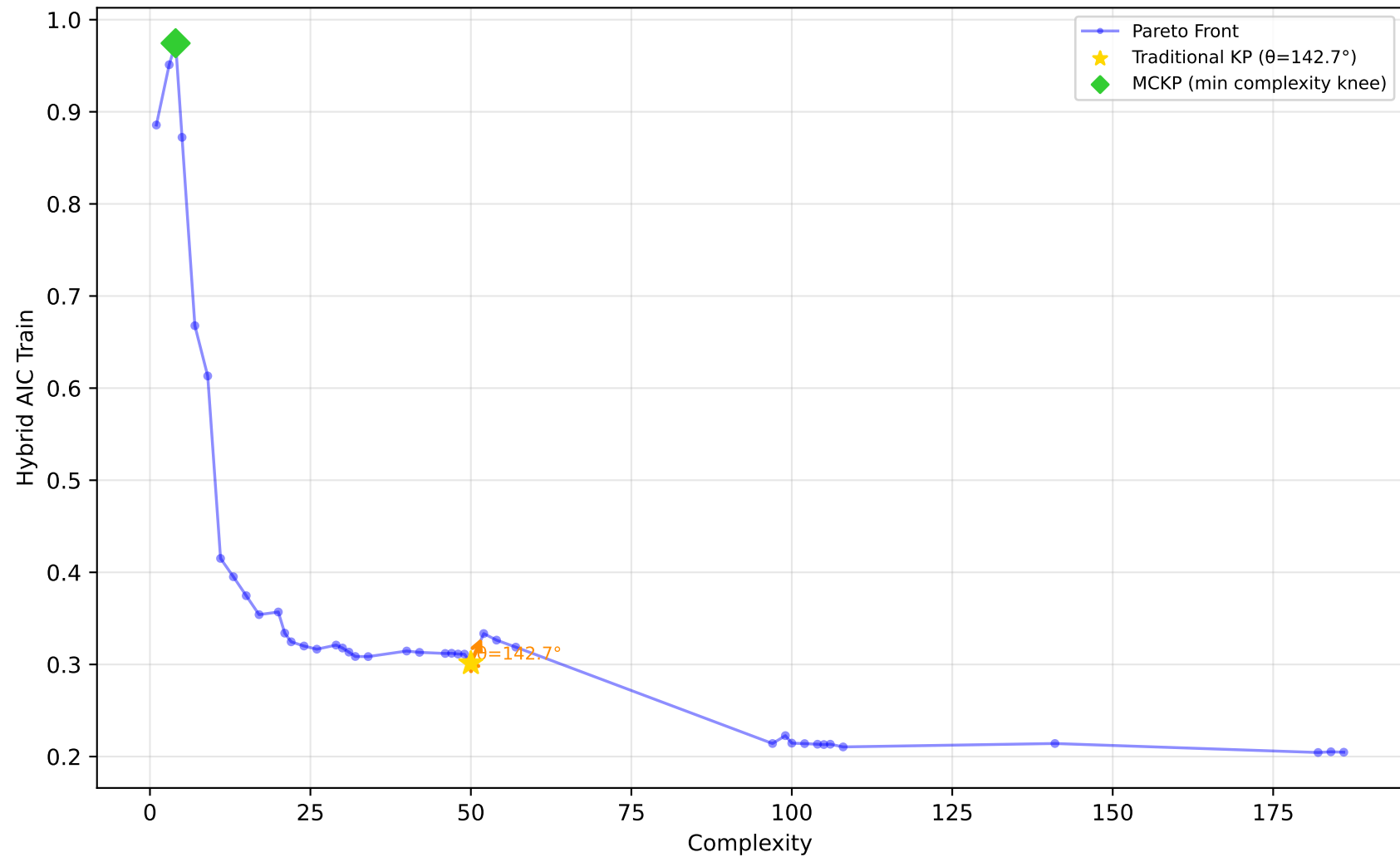
227_cpu_small - Run 15 - MVP - Hybrid AIC Train \lambda_1=0.80, \bar{\lambda}_2=0.20, \lambda_3=0.00 | Difficulty: 1.00 | Method: hmr
