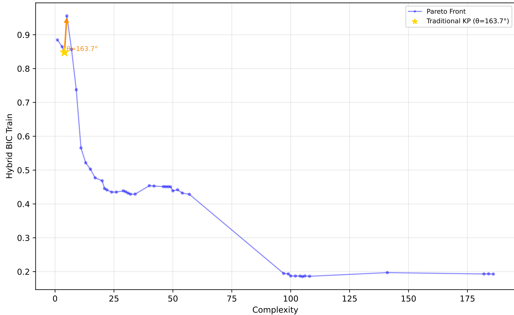
227_cpu_small - Run 15 - MVP - Hybrid BIC Train \lambda_1=0.00, \bar{\lambda}_2=0.90, \lambda_3=0.10 | Difficulty: 1.00 | Method: hmr
