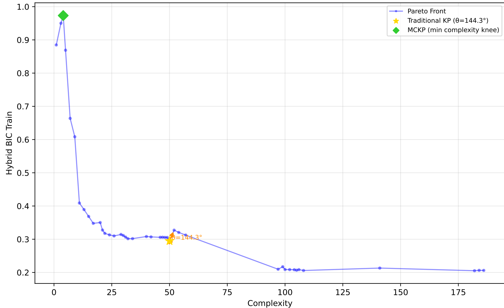
227_cpu_small - Run 15 - MVP - Hybrid BIC Train \lambda_1=0.80, \bar{\lambda}_2=0.20, \lambda_3=0.00 | Difficulty: 1.00 | Method: hmr
