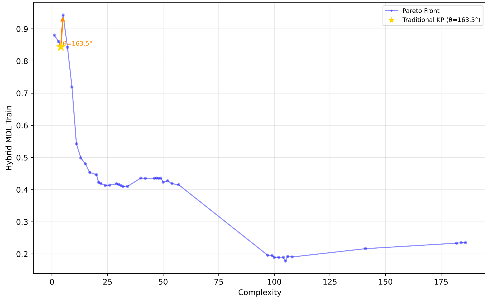
227_cpu_small - Run 15 - MVP - Hybrid MDL Train \lambda_1=0.00, \lambda_2=0.90, \lambda_3=0.10 | Difficulty: 1.00 | Method: hmr
