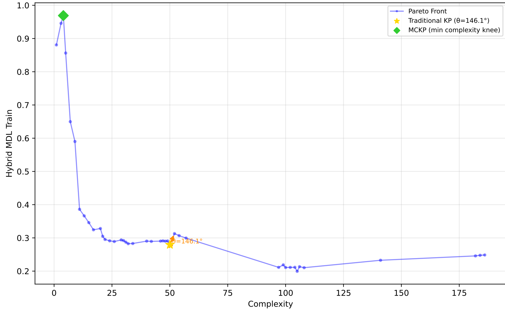
227_cpu_small - Run 15 - MVP - Hybrid MDL Train \lambda_1=0.80, \lambda_2=0.20, \lambda_3=0.00 | Difficulty: 1.00 | Method: hmr
