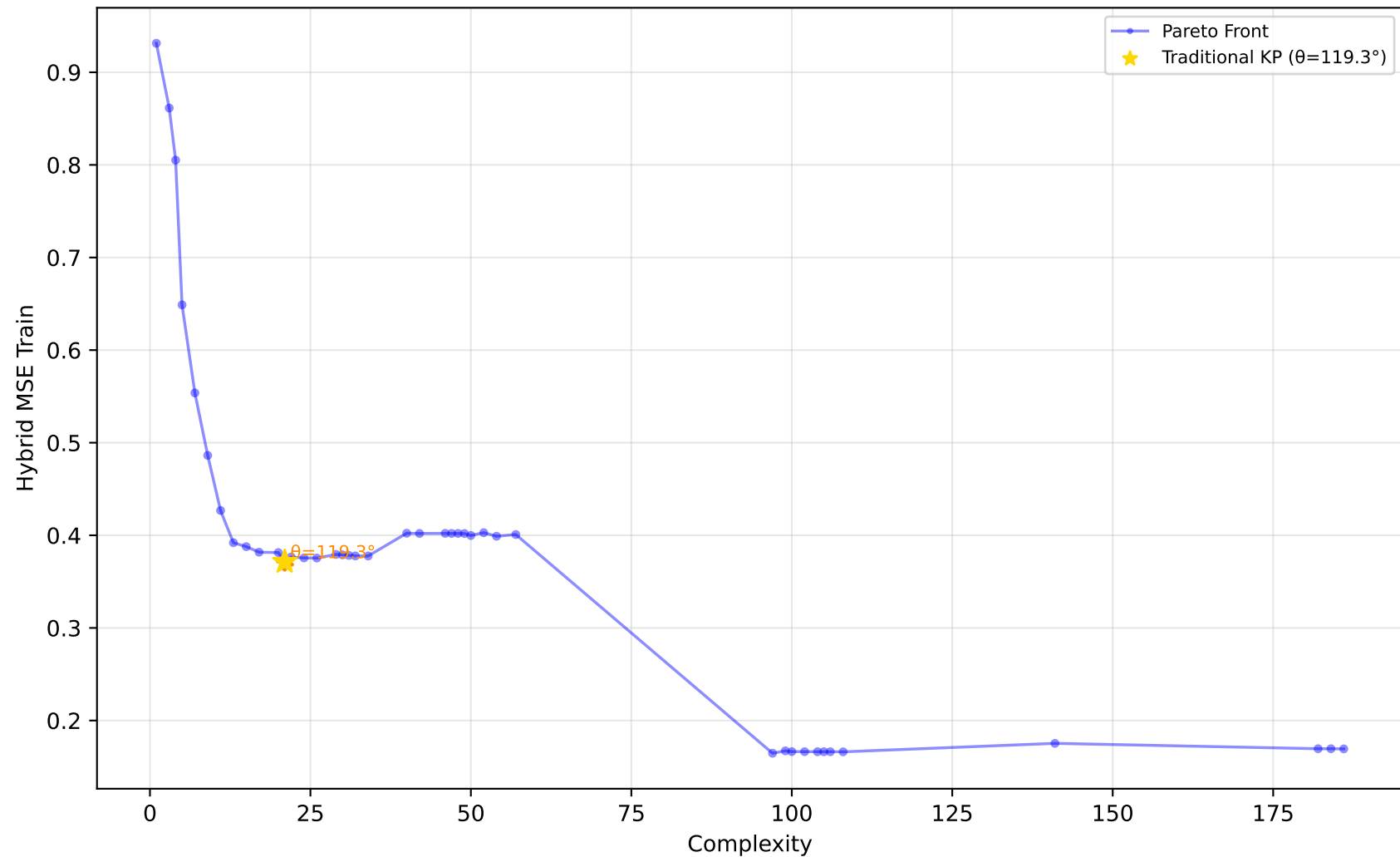
227_cpu_small - Run 15 - MVP - Hybrid MSE Train \lambda_1=0.00, \lambda_2=0.90, \lambda_3=0.10 | Difficulty: 1.00 | Method: hmr
