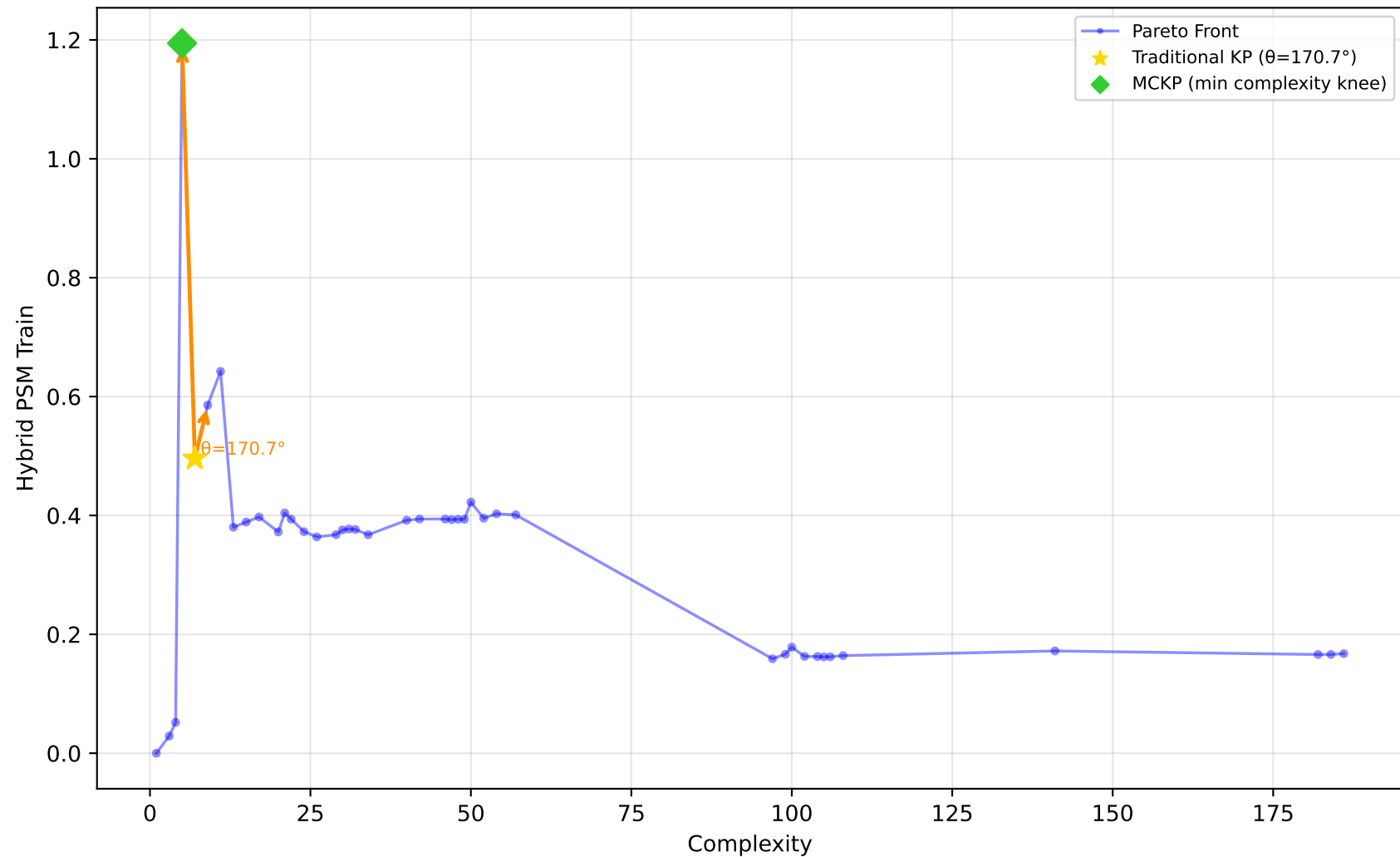
227_cpu_small - Run 15 - MVP - Hybrid PSM Train \lambda_1=0.00, \lambda_2=0.90, \lambda_3=0.10 | Difficulty: 1.00 | Method: hmr
