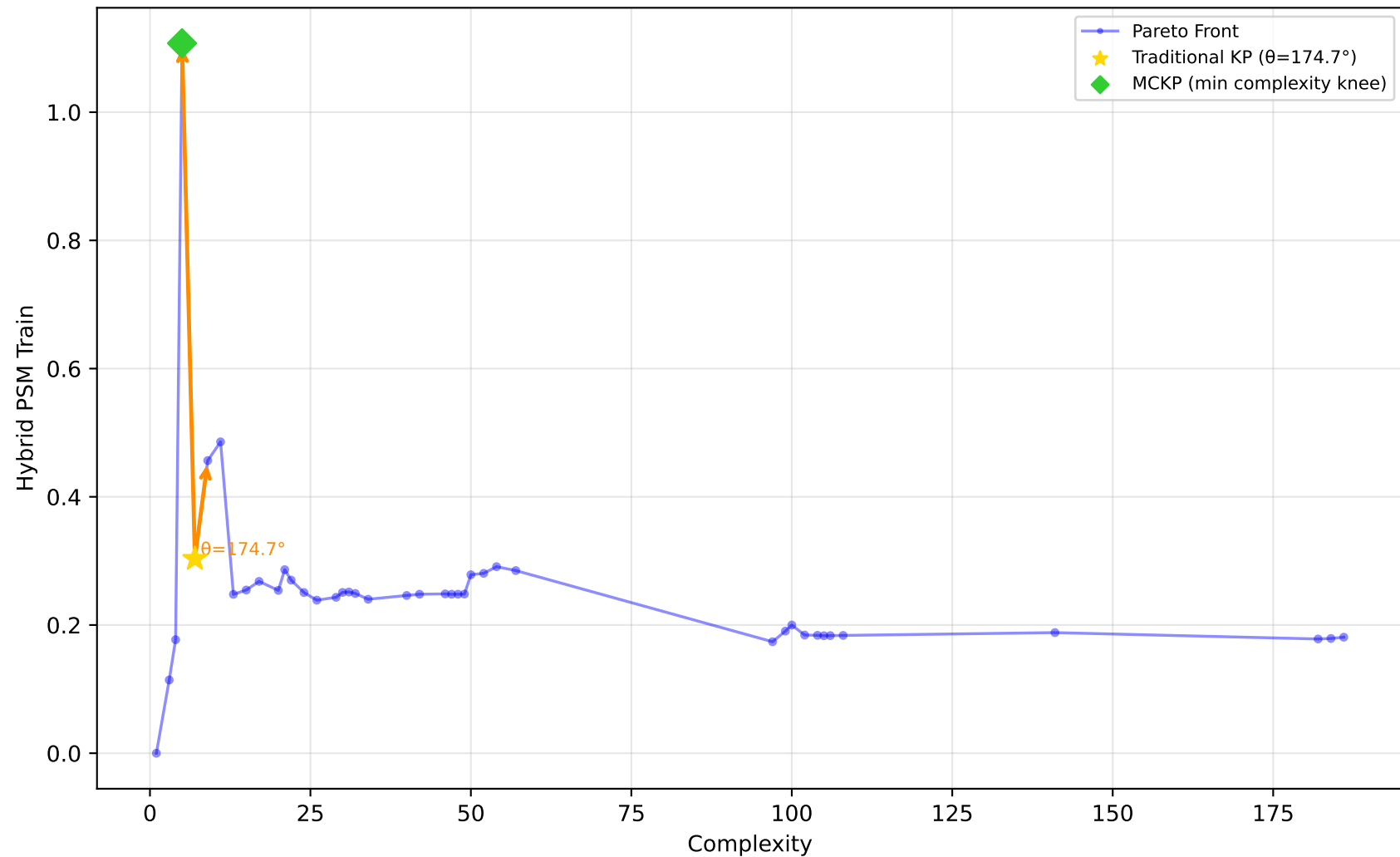
227_cpu_small - Run 15 - MVP - Hybrid PSM Train \lambda_1=0.80, \lambda_2=0.20, \lambda_3=0.00 | Difficulty: 1.00 | Method: hmr
