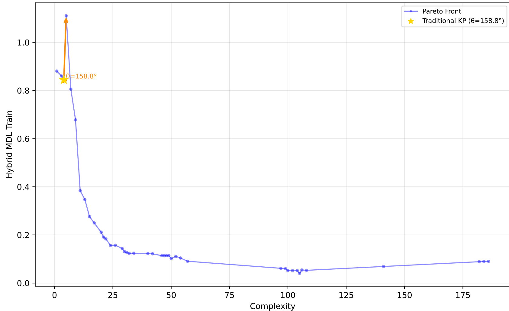
227_cpu_small - Run 15 - SVP - Hybrid MDL Train \lambda_1=0.00, \lambda_2=0.80, \lambda_3=0.30 | Difficulty: 1.00 | Method: hmr
