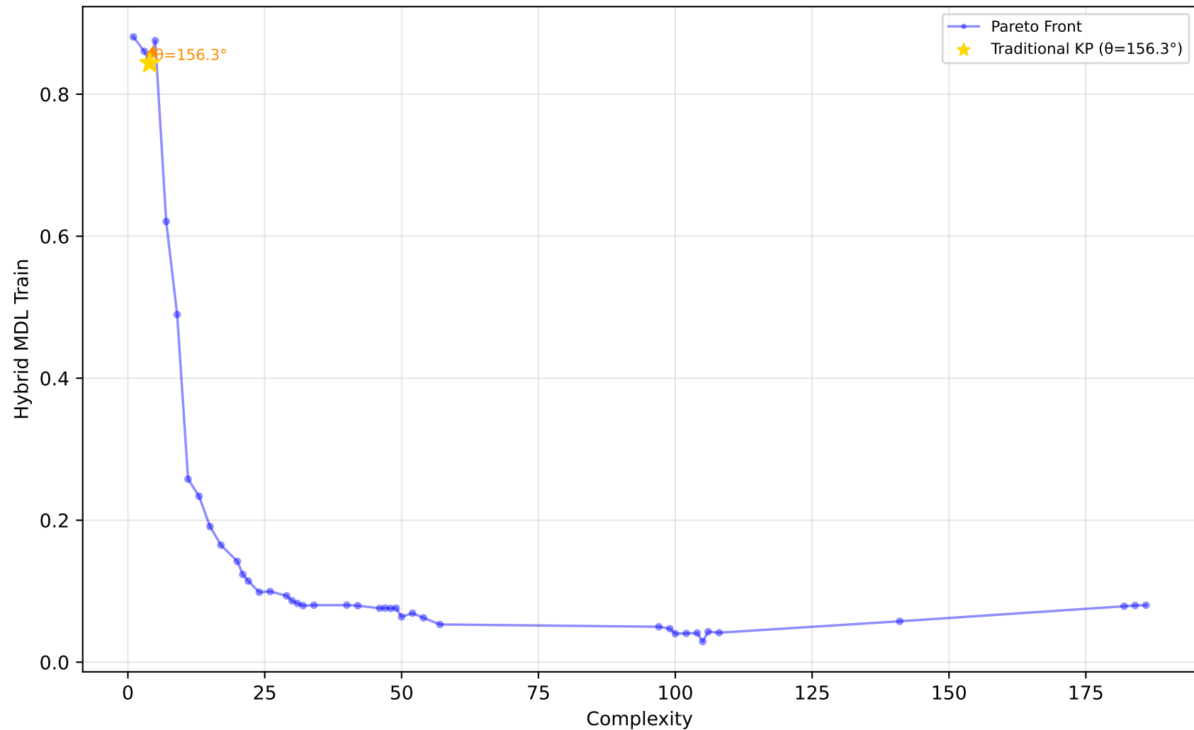
227_cpu_small - Run 15 - SVP - Hybrid MDL Train \lambda_1=0.00, \lambda_2=1.00, \lambda_3=0.00 | Difficulty: 1.00 | Method: hmr
