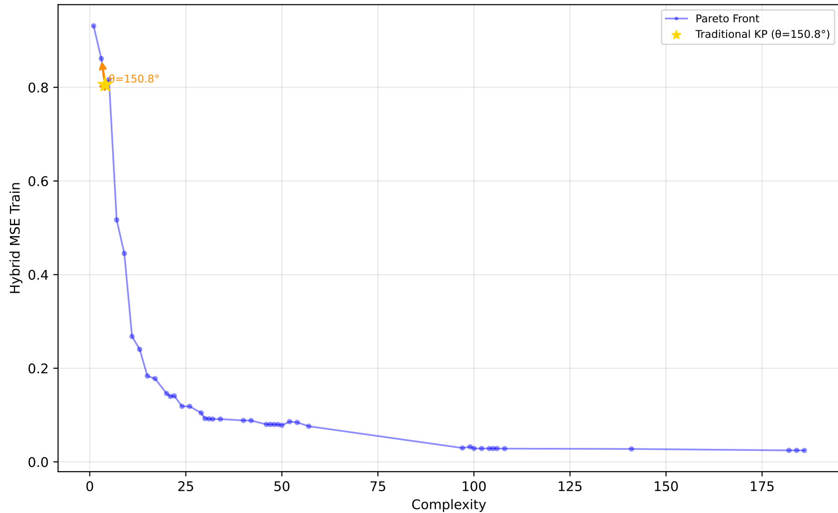
227_cpu_small - Run 15 - SVP - Hybrid MSE Train \lambda_1=0.00, \lambda_2=0.80, \lambda_3=0.30 | Difficulty: 1.00 | Method: hmr
