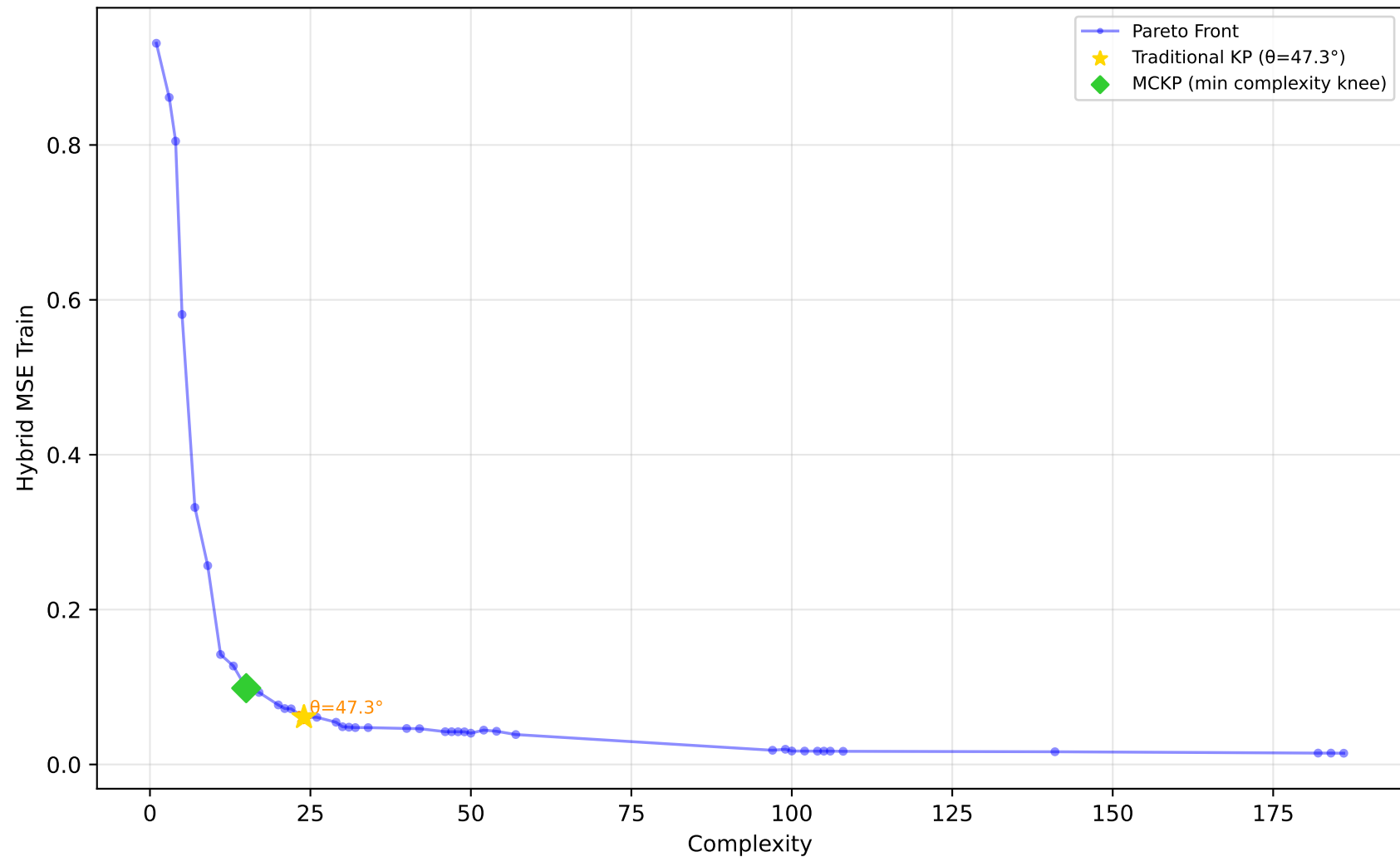
227_cpu_small - Run 15 - SVP - Hybrid MSE Train \lambda_1=0.00, \lambda_2=1.00, \lambda_3=0.00 | Difficulty: 1.00 | Method: hmr
