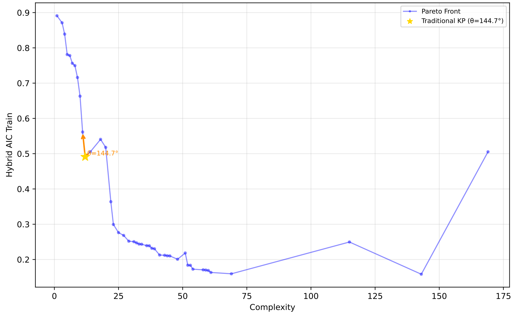
227_cpu_small - Run 16 - MVP - Hybrid AIC Train \lambda_1=0.00, \bar{\lambda}_2=0.90, \lambda_3=0.10 | Difficulty: 1.00 | Method: hmr
