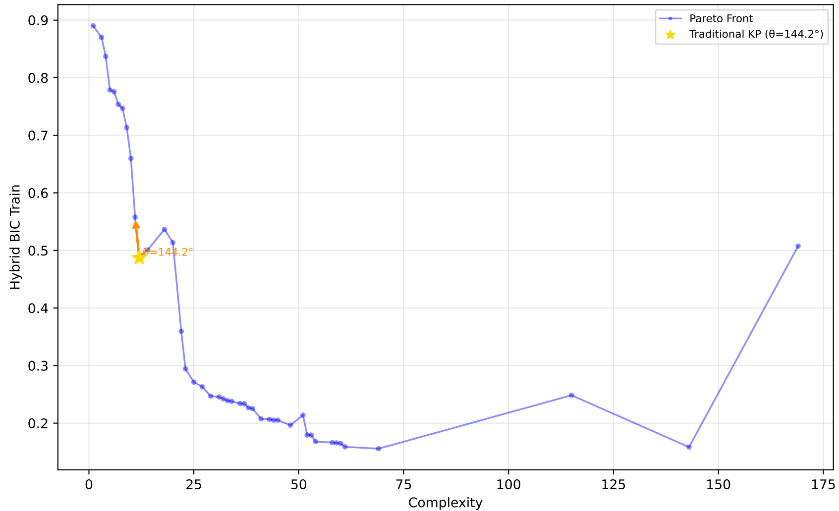
227_cpu_small - Run 16 - MVP - Hybrid BIC Train \lambda_1=0.00, \bar{\lambda}_2=0.90, \lambda_3=0.10 | Difficulty: 1.00 | Method: hmr
