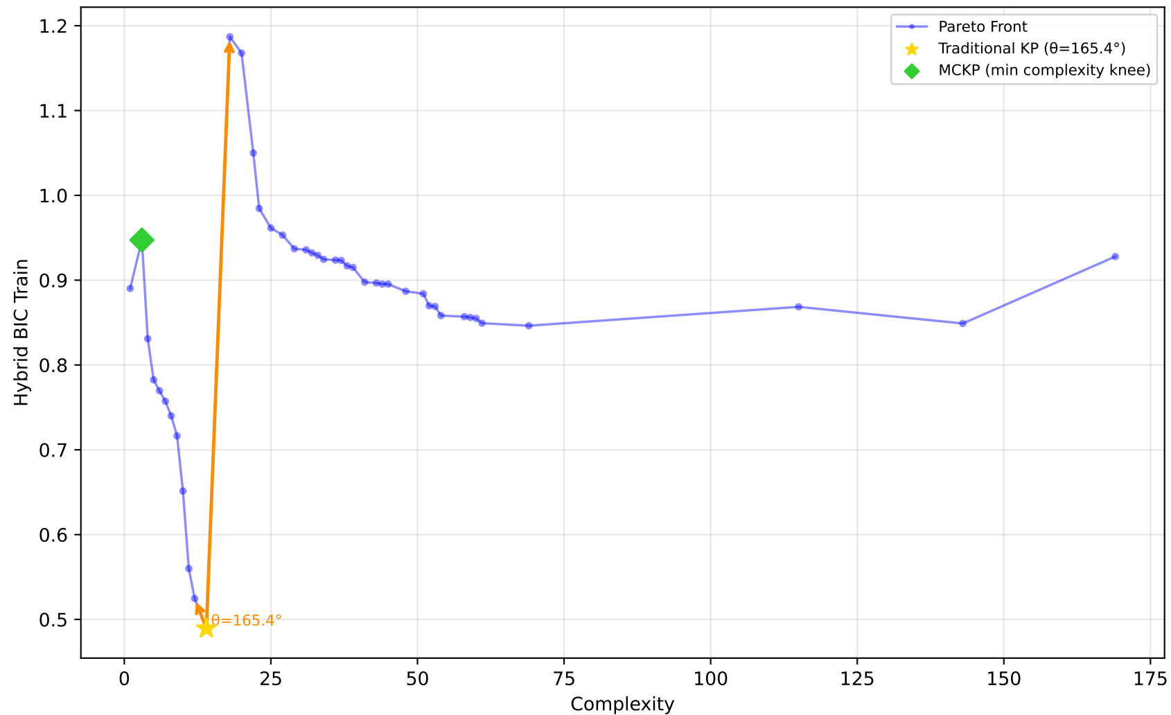
227_cpu_small - Run 16 - MVP - Hybrid BIC Train \lambda_1=0.80, \bar{\lambda}_2=0.20, \lambda_3=0.00 | Difficulty: 1.00 | Method: hmr
