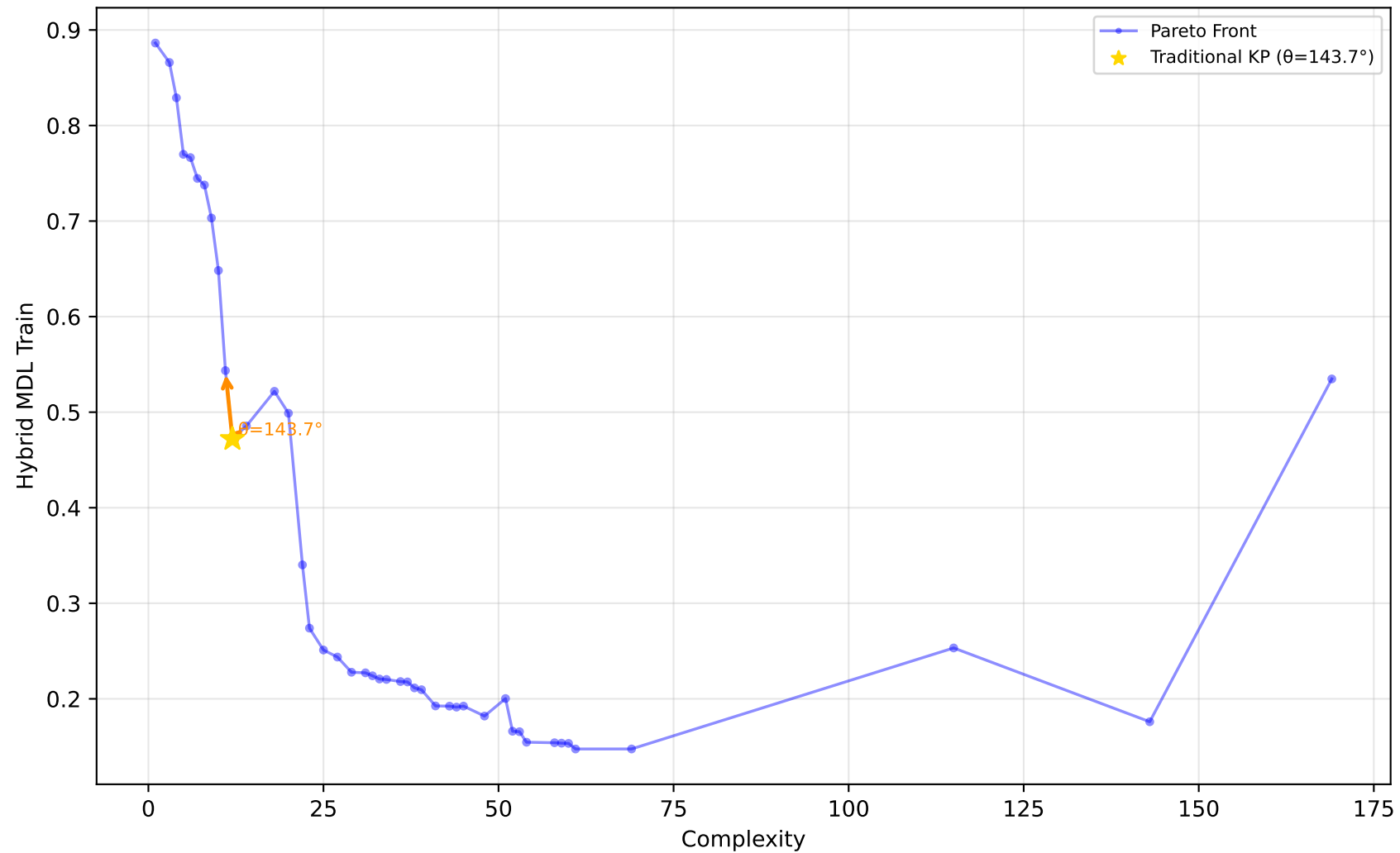
227_cpu_small - Run 16 - MVP - Hybrid MDL Train \lambda_1=0.00, \lambda_2=0.90, \lambda_3=0.10 | Difficulty: 1.00 | Method: hmr
