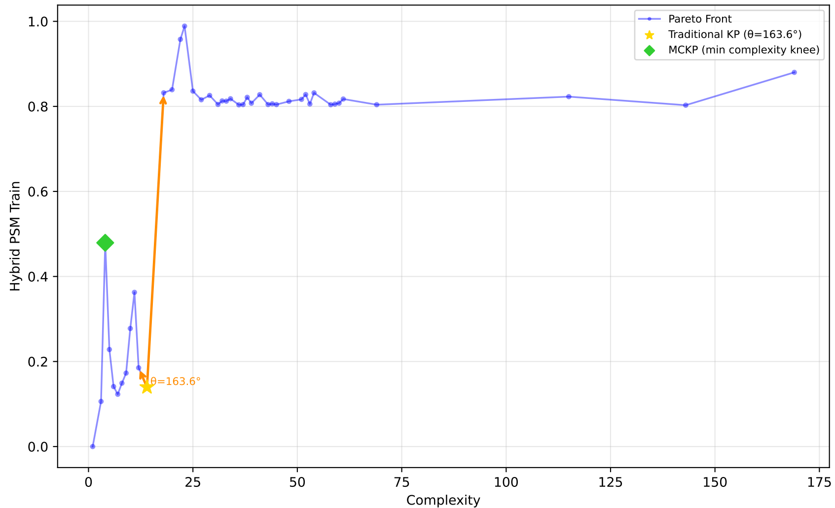
227_cpu_small - Run 16 - MVP - Hybrid PSM Train \lambda_1=0.80, \lambda_2=0.20, \lambda_3=0.00 | Difficulty: 1.00 | Method: hmr
