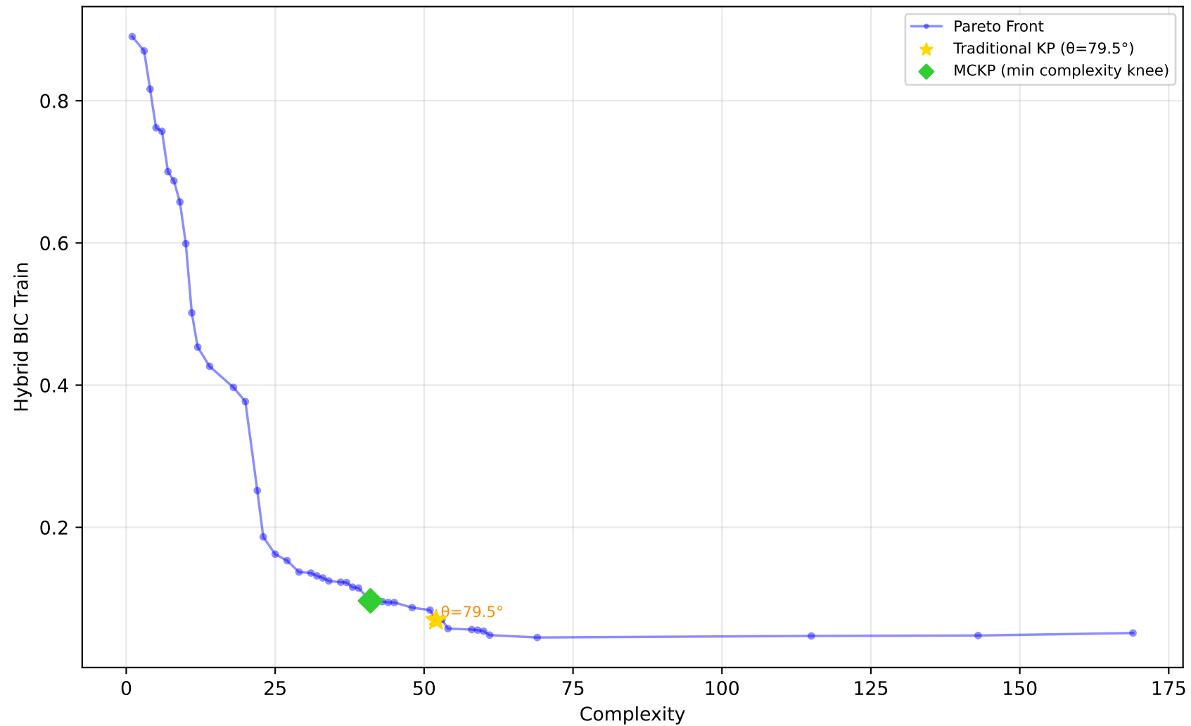
227_cpu_small - Run 16 - SVP - Hybrid BIC Train \lambda_1=0.00, \lambda_2=1.00, \lambda_3=0.00 | Difficulty: 1.00 | Method: hmr
