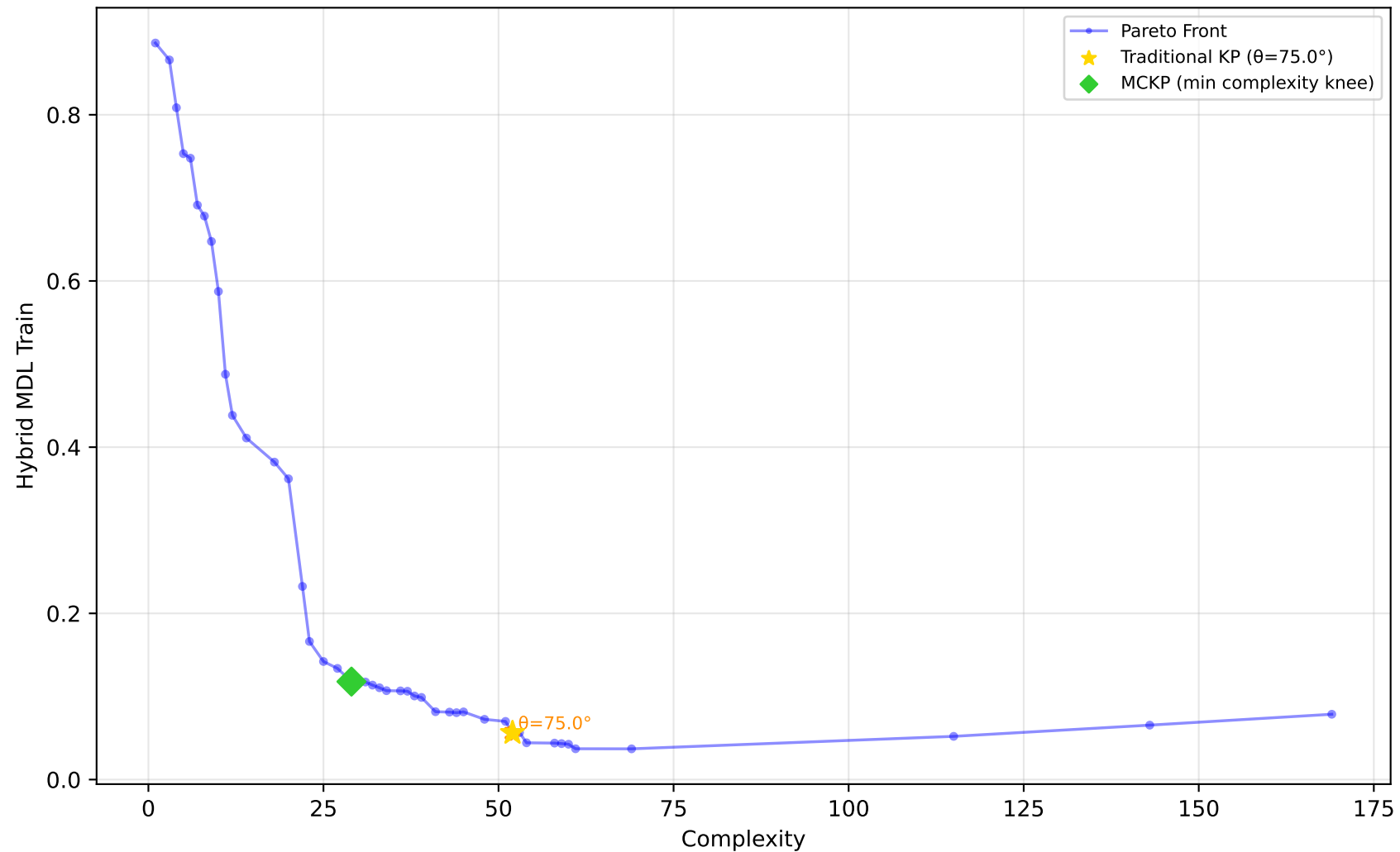
227_cpu_small - Run 16 - SVP - Hybrid MDL Train \lambda_1=0.00, \lambda_2=1.00, \lambda_3=0.00 | Difficulty: 1.00 | Method: hmr
