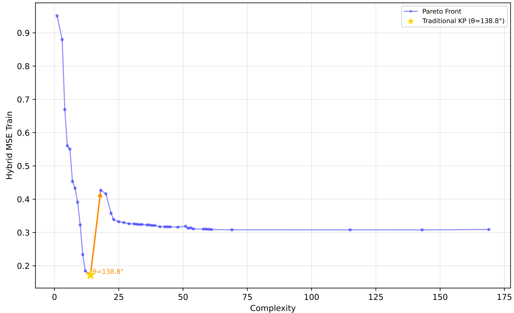
227_cpu_small - Run 16 - SVP - Hybrid MSE Train \lambda_1=0.00, \lambda_2=0.80, \lambda_3=0.30 | Difficulty: 1.00 | Method: hmr
