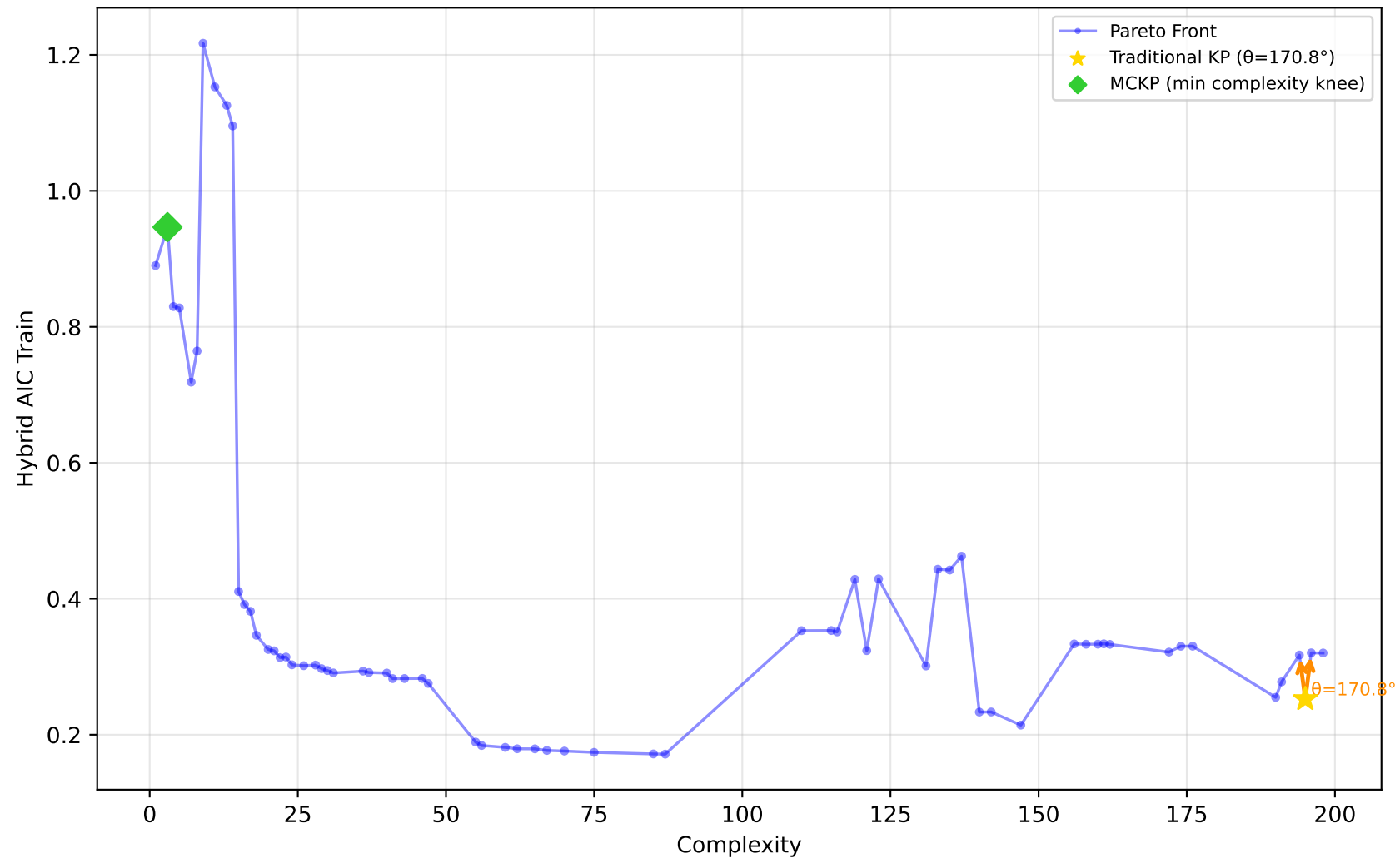
227_cpu_small - Run 17 - MVP - Hybrid AIC Train \lambda_1=0.80, \bar{\lambda}_2=0.20, \lambda_3=0.00 | Difficulty: 1.00 | Method: hmr
