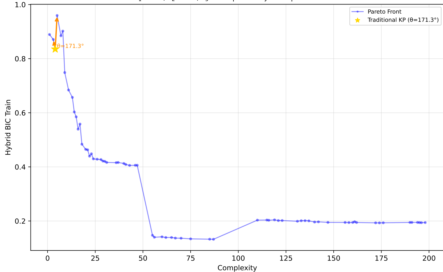
227_cpu_small - Run 17 - MVP - Hybrid BIC Train \lambda_1=0.00, \bar{\lambda}_2=0.90, \lambda_3=0.10 | Difficulty: 1.00 | Method: hmr
