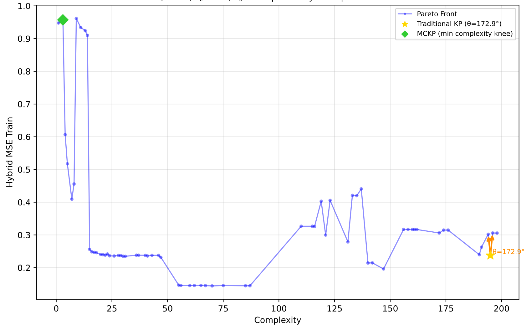
227_cpu_small - Run 17 - MVP - Hybrid MSE Train \lambda_1=0.80, \lambda_2=0.20, \lambda_3=0.00 | Difficulty: 1.00 | Method: hmr
