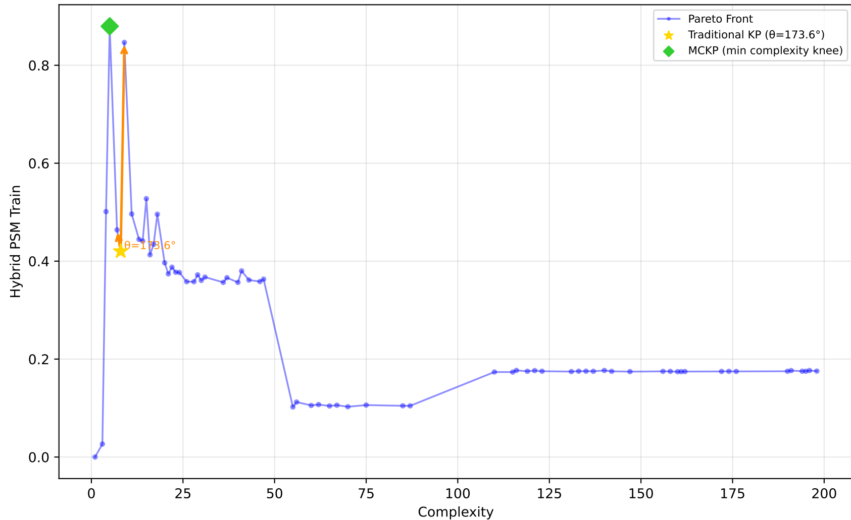
227_cpu_small - Run 17 - MVP - Hybrid PSM Train \lambda_1=0.00, \lambda_2=0.90, \lambda_3=0.10 | Difficulty: 1.00 | Method: hmr
