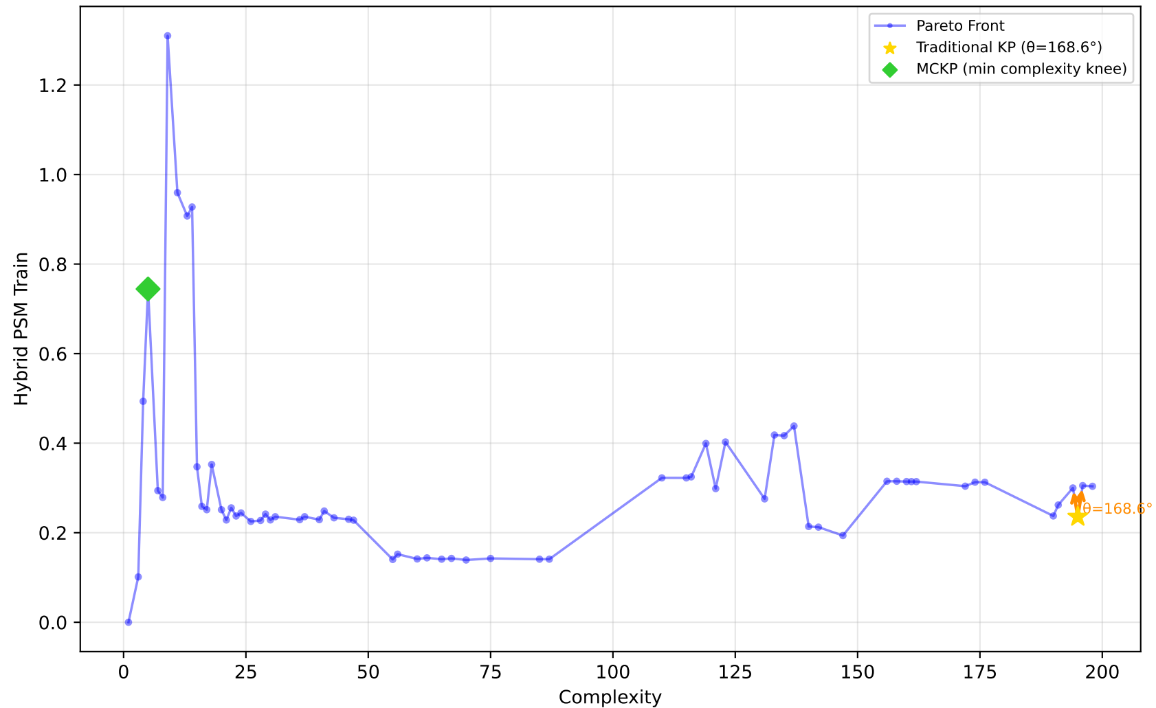
227_cpu_small - Run 17 - MVP - Hybrid PSM Train \lambda_1=0.80, \lambda_2=0.20, \lambda_3=0.00 | Difficulty: 1.00 | Method: hmr
