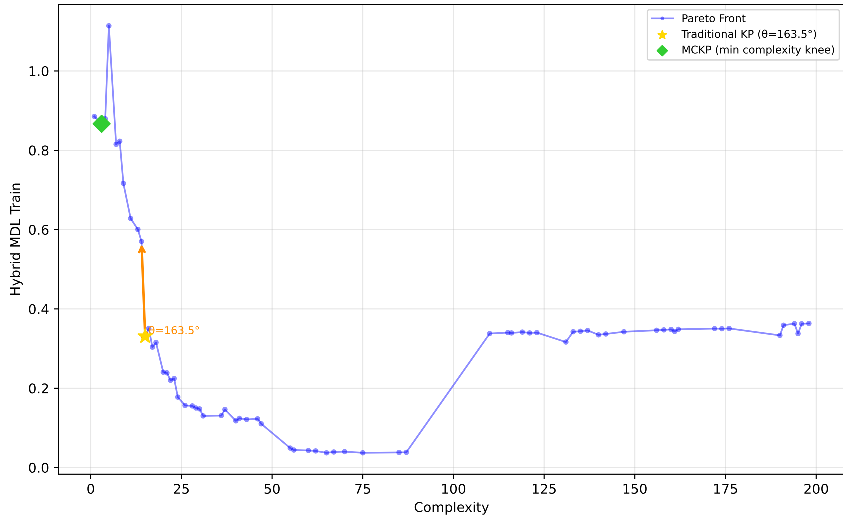
227_cpu_small - Run 17 - SVP - Hybrid MDL Train \lambda_1=0.00, \lambda_2=0.80, \lambda_3=0.30 | Difficulty: 1.00 | Method: hmr
