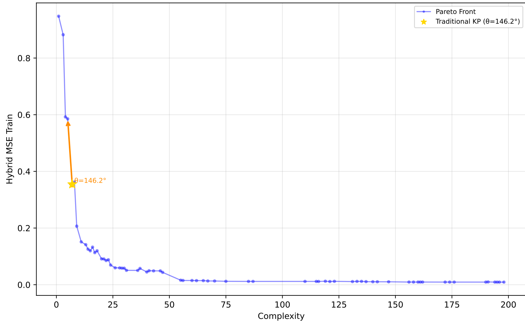
227_cpu_small - Run 17 - SVP - Hybrid MSE Train \lambda_1=0.00, \lambda_2=1.00, \lambda_3=0.00 | Difficulty: 1.00 | Method: hmr
