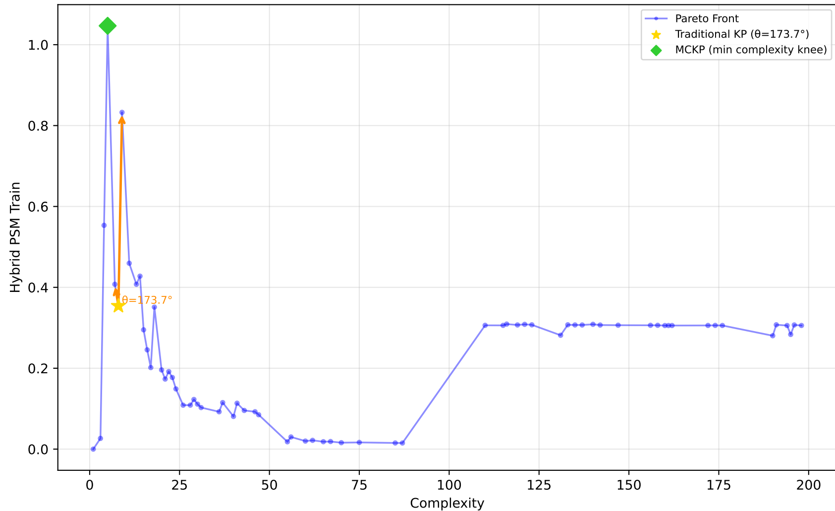
227_cpu_small - Run 17 - SVP - Hybrid PSM Train \lambda_1=0.00, \lambda_2=0.80, \lambda_3=0.30 | Difficulty: 1.00 | Method: hmr
