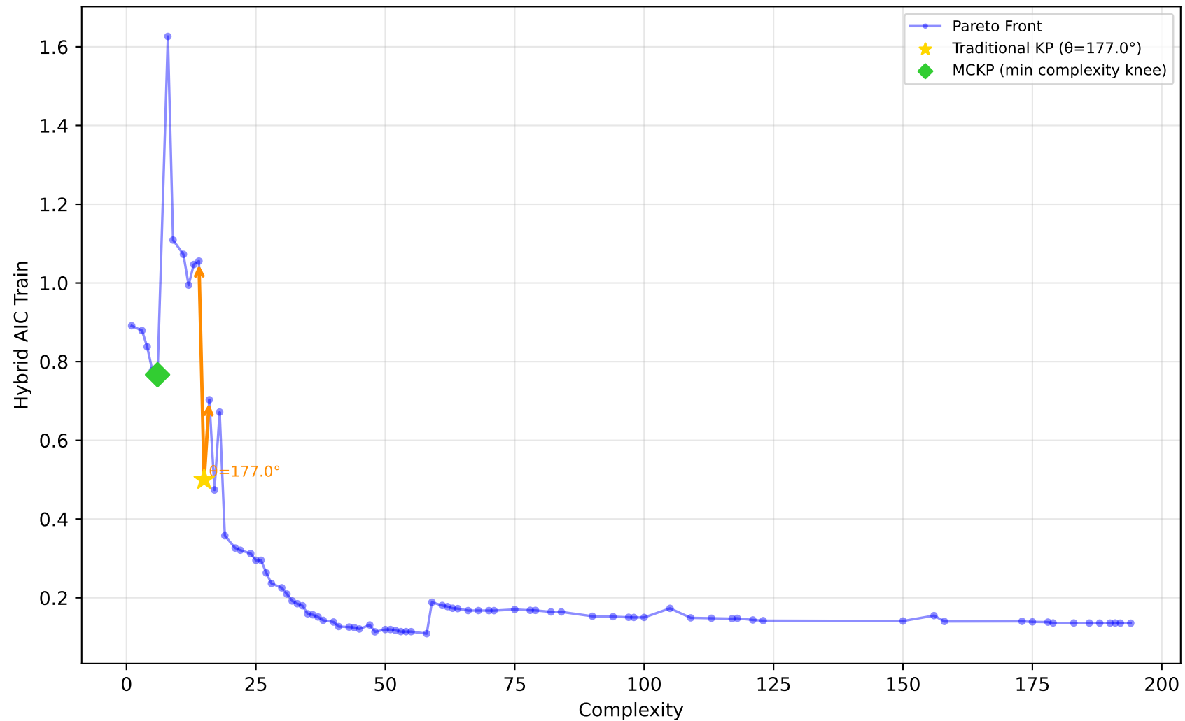
227_cpu_small - Run 18 - MVP - Hybrid AIC Train \lambda_1=0.00, \bar{\lambda}_2=0.90, \lambda_3=0.10 | Difficulty: 1.00 | Method: hmr
