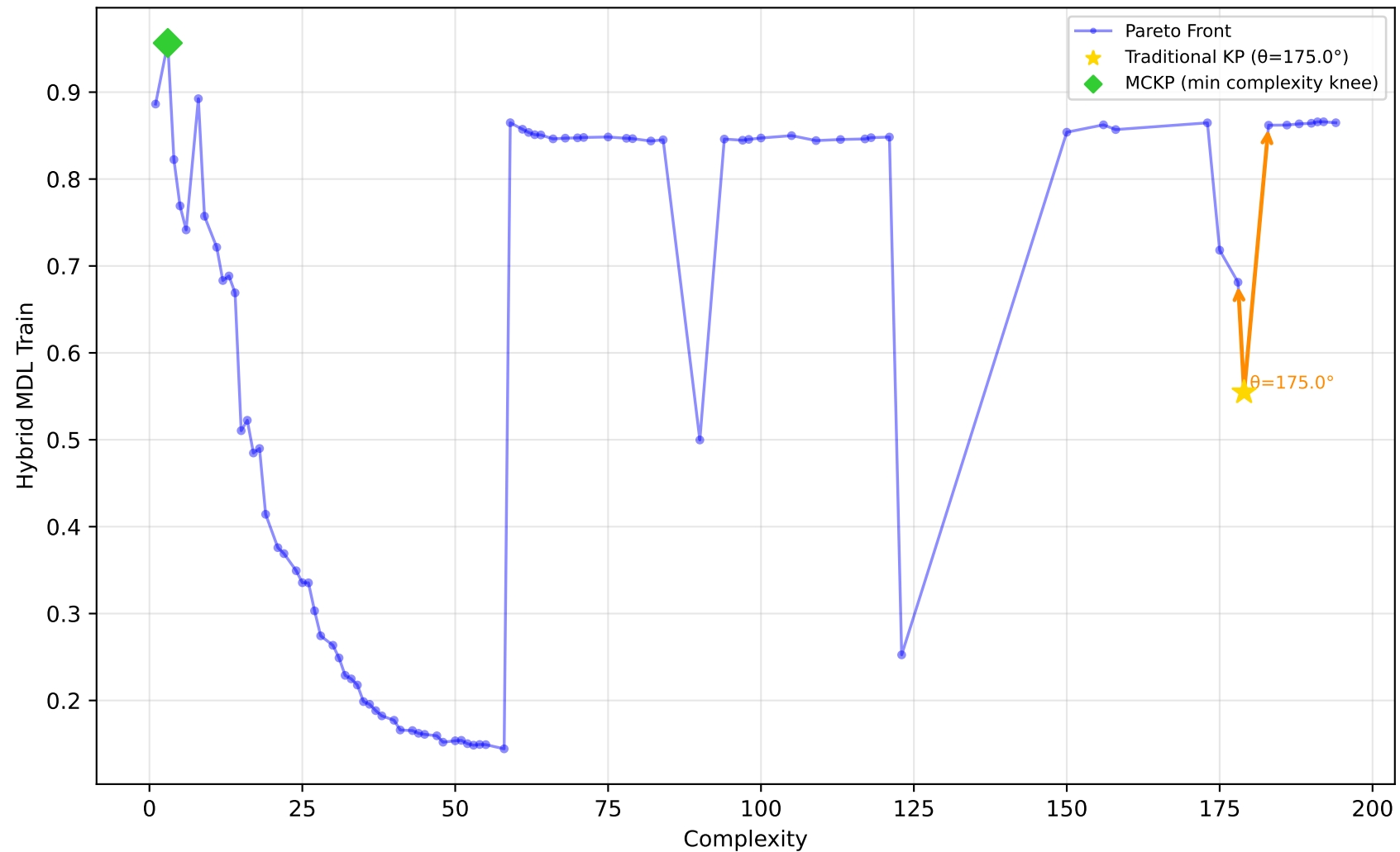
227_cpu_small - Run 18 - MVP - Hybrid MDL Train \lambda_1=0.80, \lambda_2=0.20, \lambda_3=0.00 | Difficulty: 1.00 | Method: hmr
