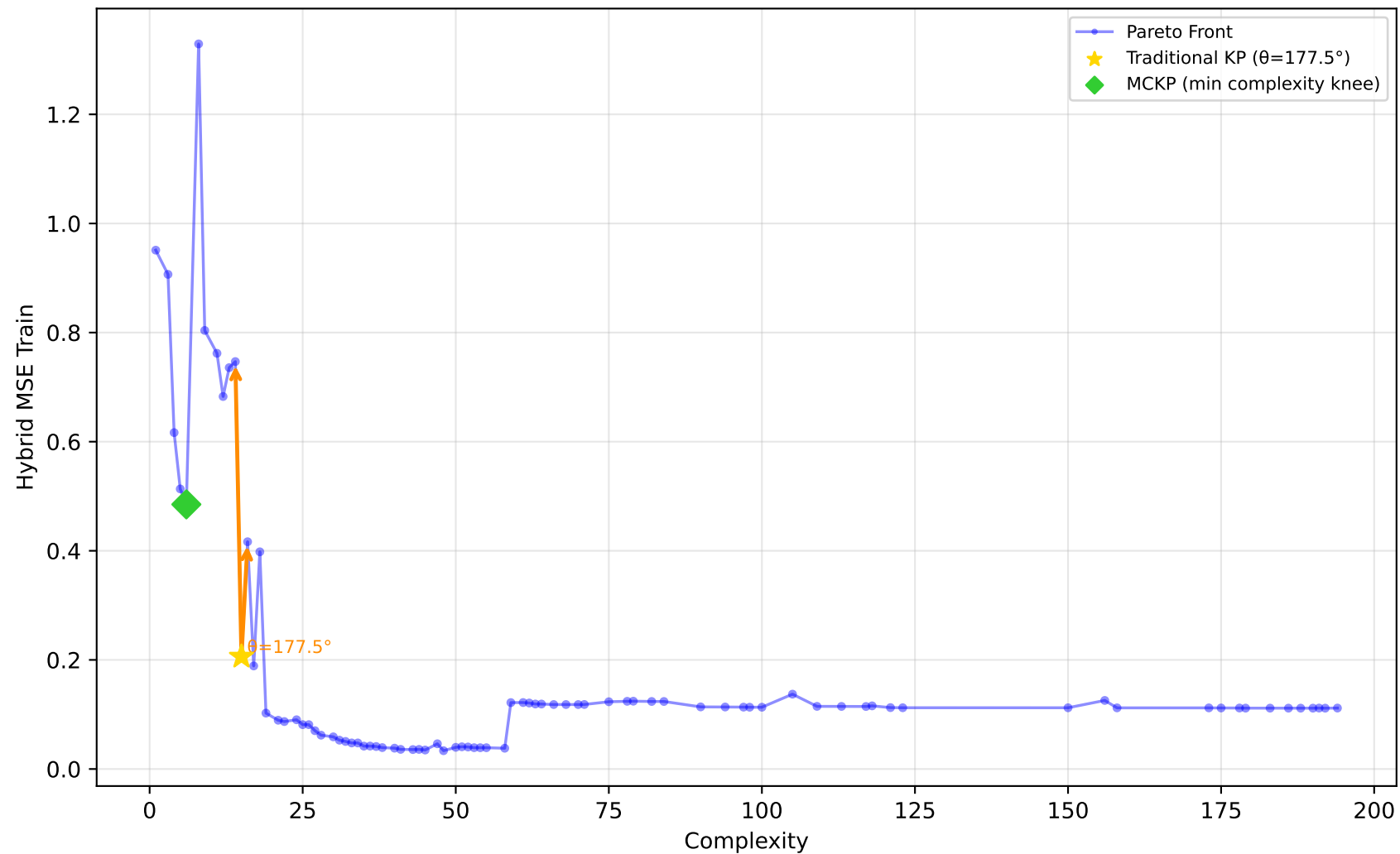
227_cpu_small - Run 18 - MVP - Hybrid MSE Train \lambda_1=0.00, \lambda_2=0.90, \lambda_3=0.10 | Difficulty: 1.00 | Method: hmr
