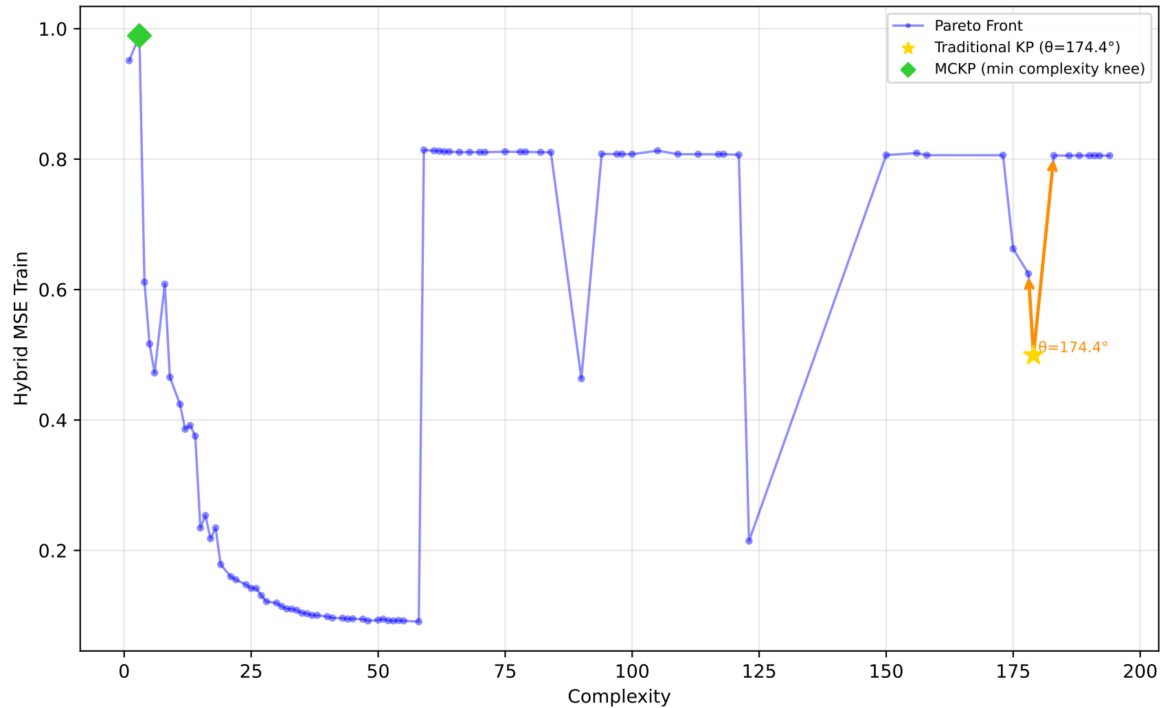
227_cpu_small - Run 18 - MVP - Hybrid MSE Train \lambda_1=0.80, \lambda_2=0.20, \lambda_3=0.00 | Difficulty: 1.00 | Method: hmr
