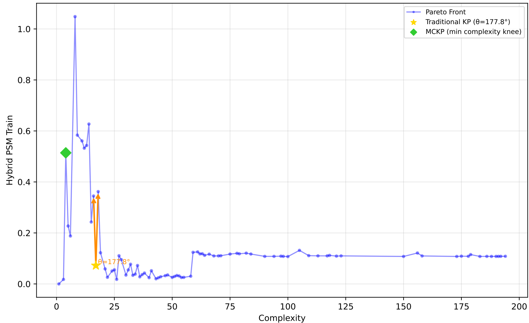
227_cpu_small - Run 18 - MVP - Hybrid PSM Train \lambda_1=0.00, \lambda_2=0.90, \lambda_3=0.10 | Difficulty: 1.00 | Method: hmr
