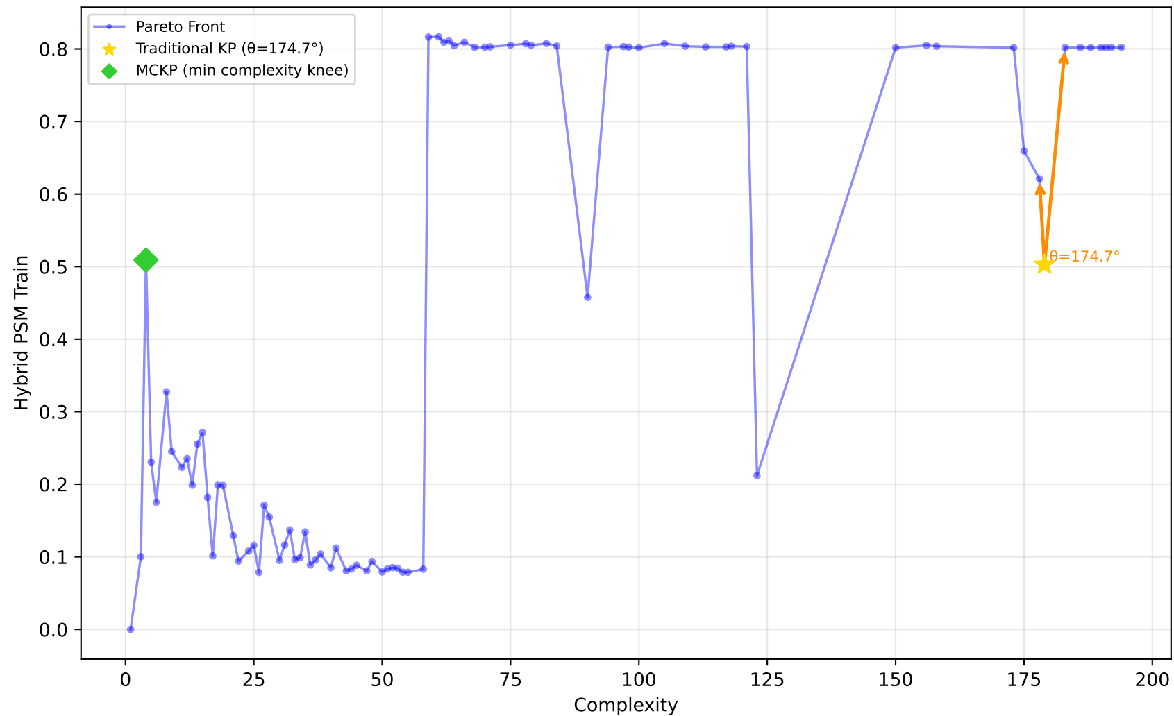
227_cpu_small - Run 18 - MVP - Hybrid PSM Train \lambda_1=0.80, \bar{\lambda}_2=0.20, \lambda_3=0.00 | Difficulty: 1.00 | Method: hmr
