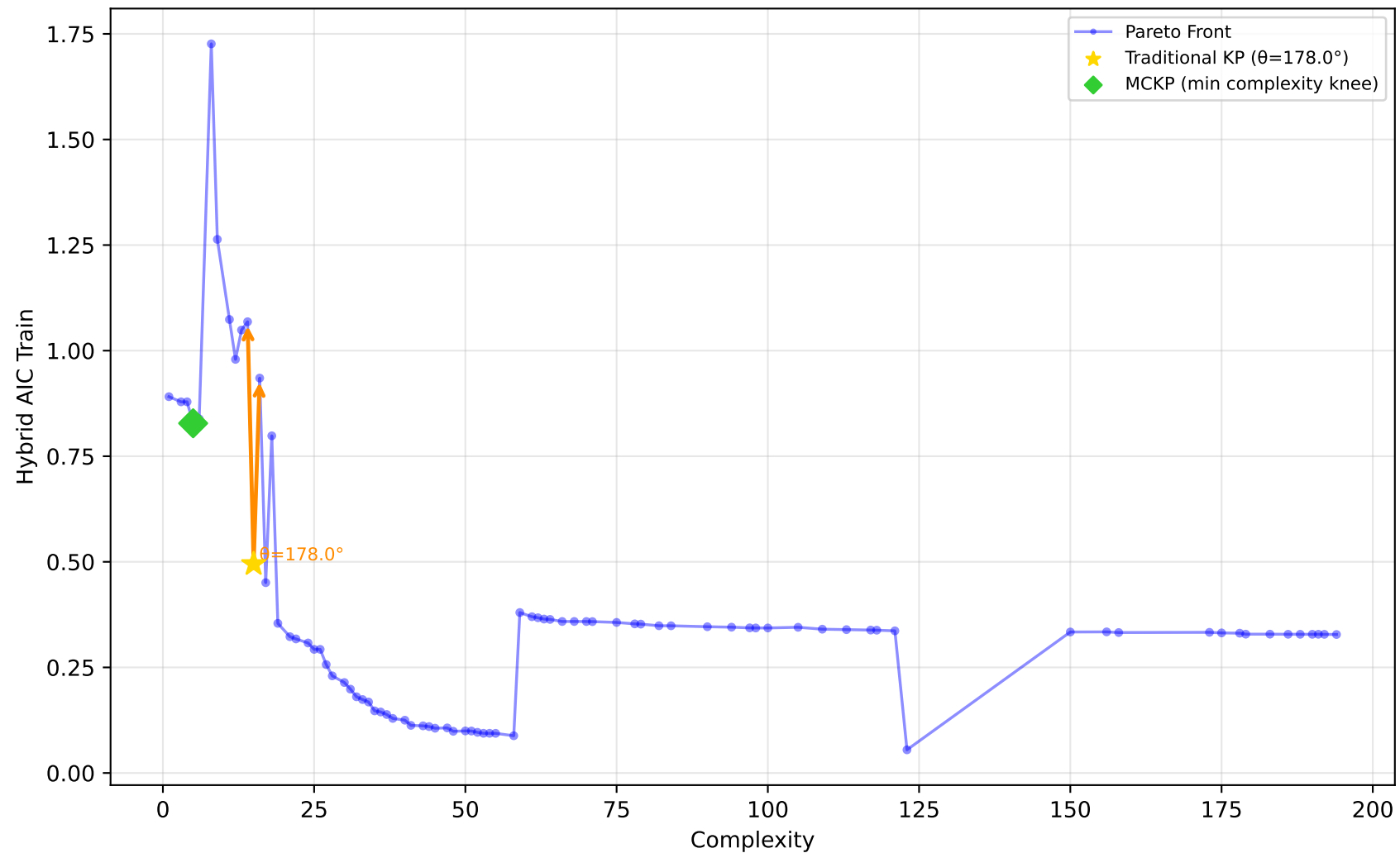
227_cpu_small - Run 18 - SVP - Hybrid AIC Train \lambda_1=0.00 , \bar{\lambda}_2=0.80 , \lambda_3=0.30 | Difficulty: 1.00 | Method: hmr
