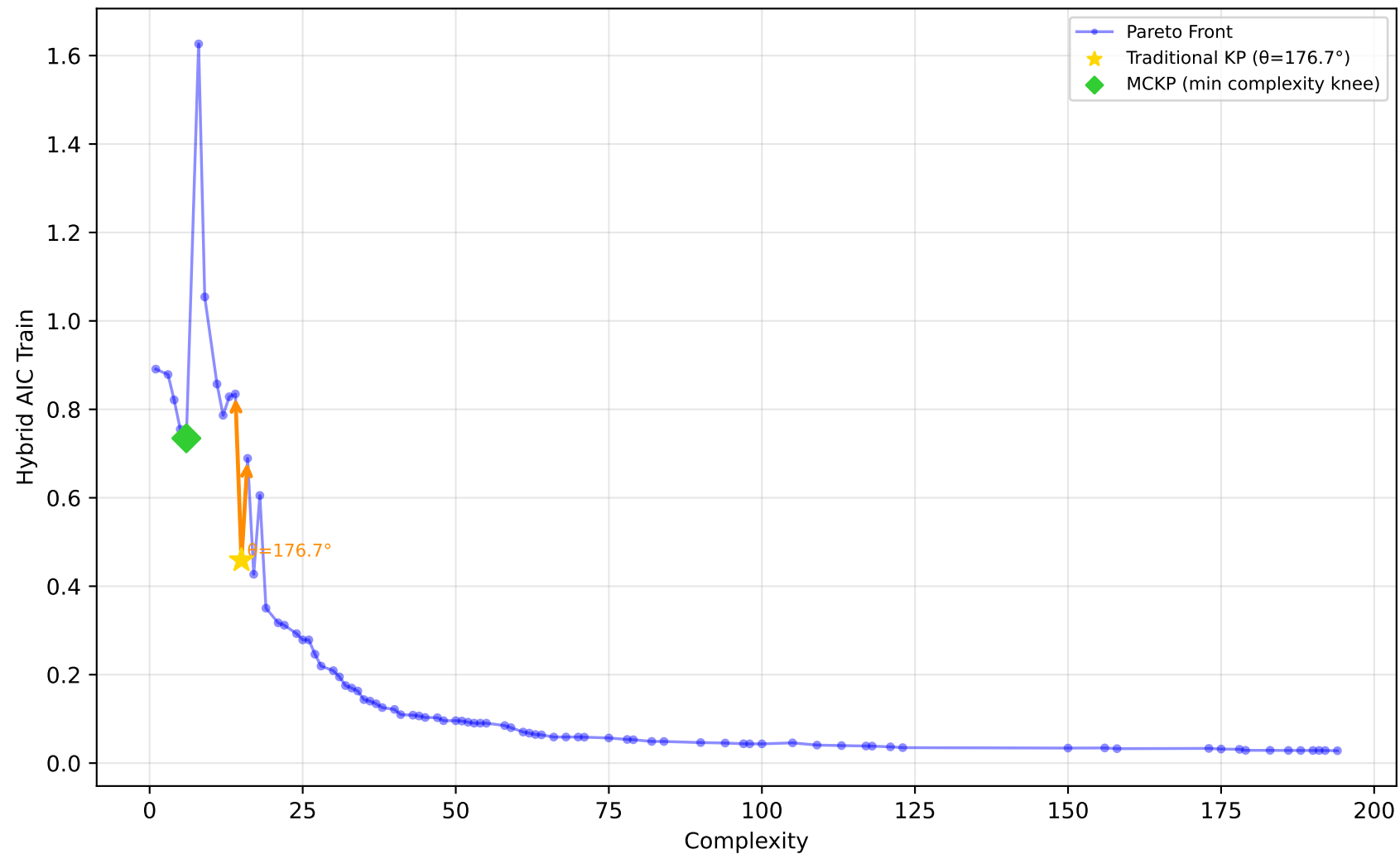
227_cpu_small - Run 18 - SVP - Hybrid AIC Train \lambda_1=0.00, \bar{\lambda}_2=1.00, \lambda_3=0.00 | Difficulty: 1.00 | Method: hmr
