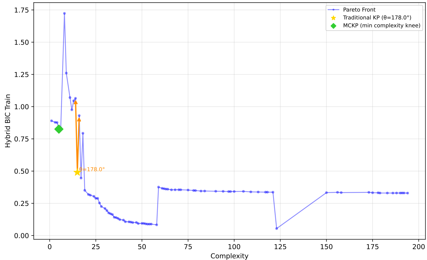
227_cpu_small - Run 18 - SVP - Hybrid BIC Train \lambda_1=0.00, \bar{\lambda}_2=0.80, \lambda_3=0.30 | Difficulty: 1.00 | Method: hmr
