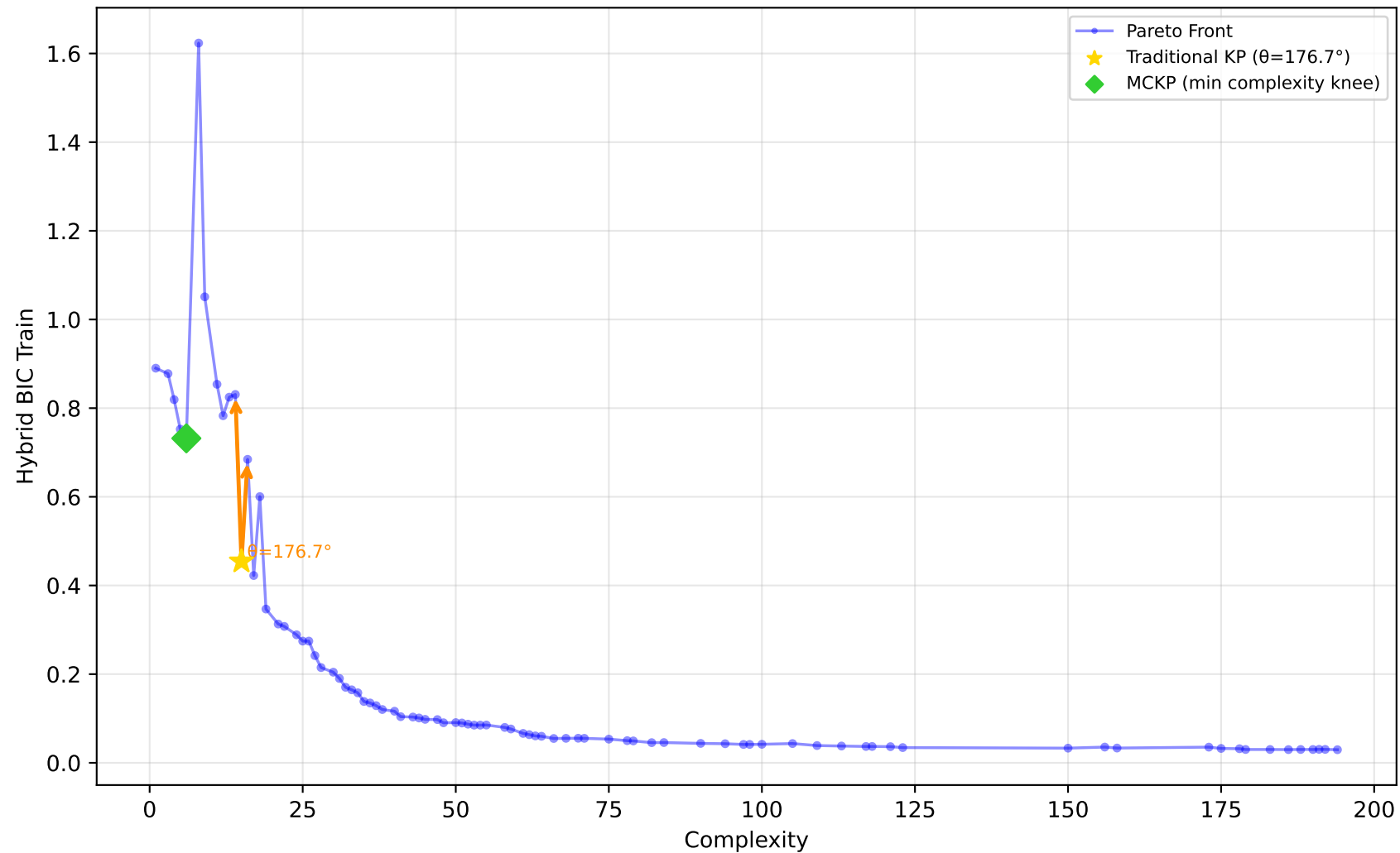
227_cpu_small - Run 18 - SVP - Hybrid BIC Train \lambda_1=0.00, \bar{\lambda}_2=1.00, \lambda_3=0.00 | Difficulty: 1.00 | Method: hmr
