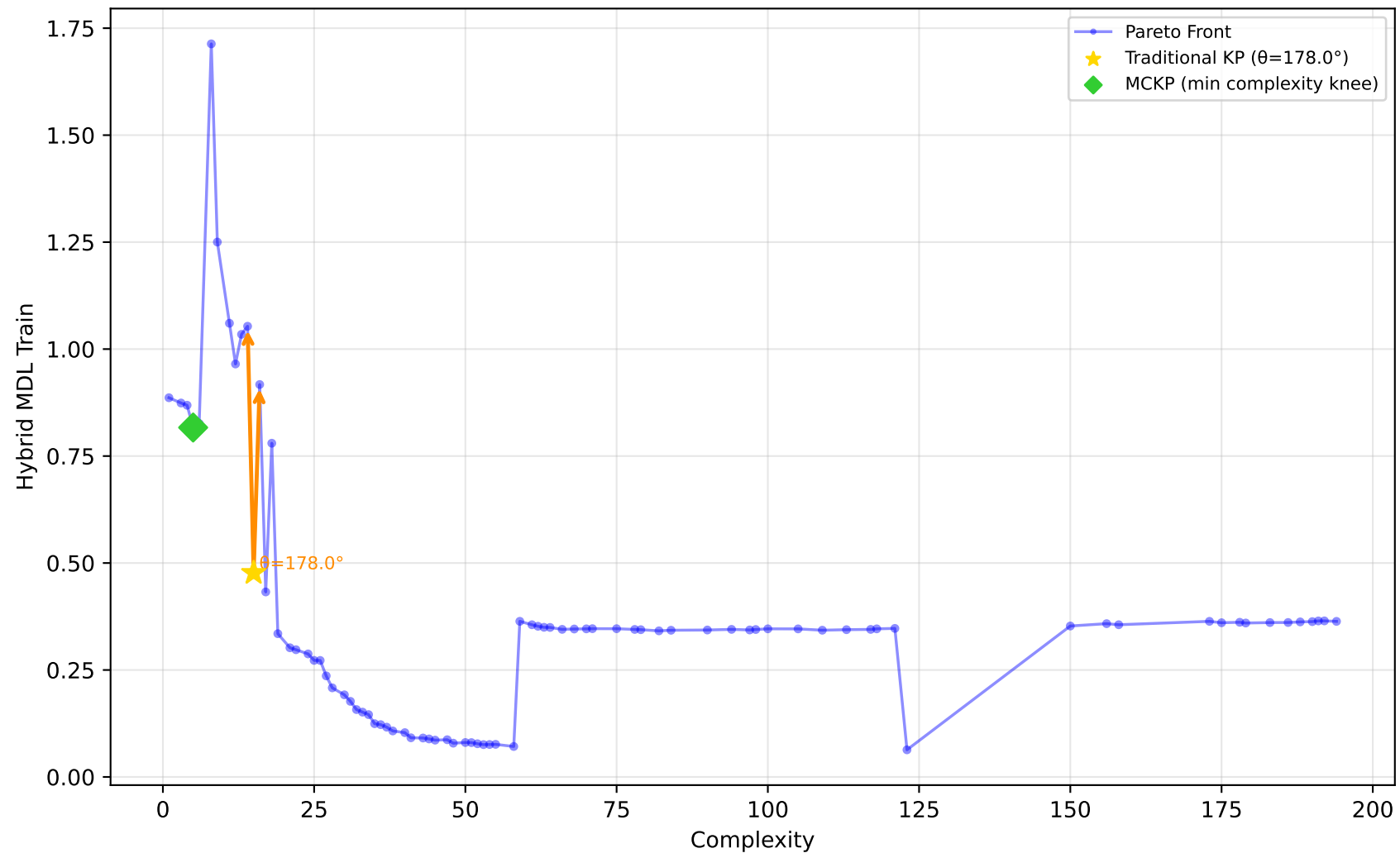
227_cpu_small - Run 18 - SVP - Hybrid MDL Train \lambda_1=0.00, \lambda_2=0.80, \lambda_3=0.30 | Difficulty: 1.00 | Method: hmr
