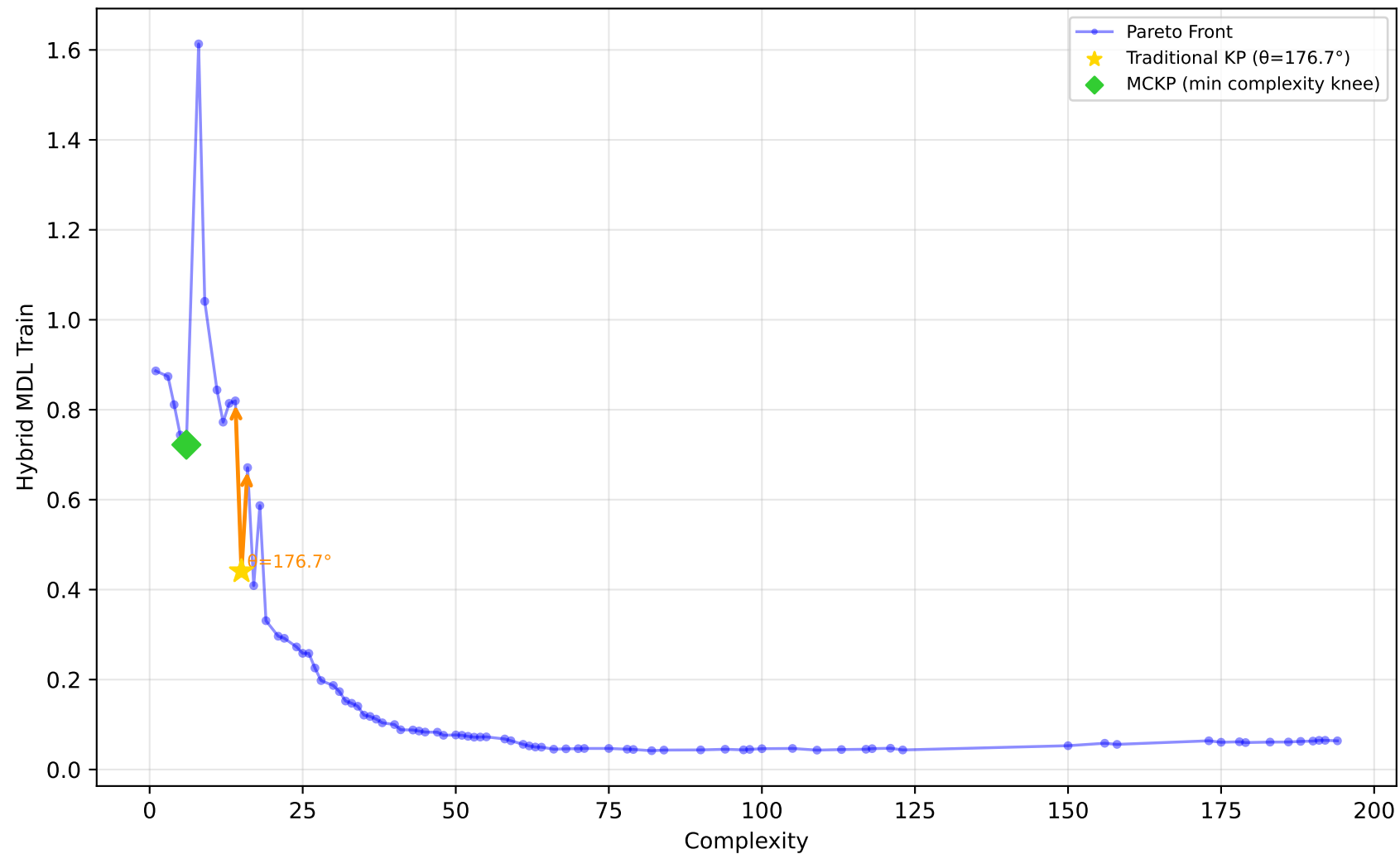
227_cpu_small - Run 18 - SVP - Hybrid MDL Train \lambda_1=0.00, \lambda_2=1.00, \lambda_3=0.00 | Difficulty: 1.00 | Method: hmr
