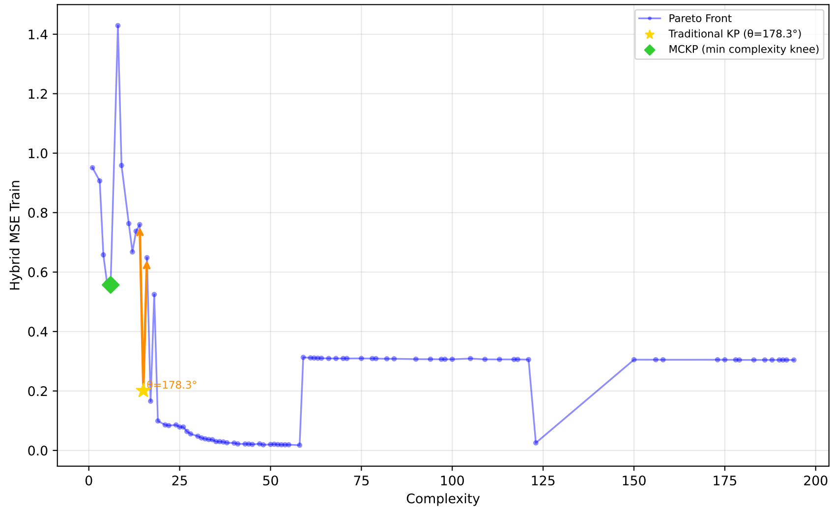
227_cpu_small - Run 18 - SVP - Hybrid MSE Train \lambda_1=0.00, \lambda_2=0.80, \lambda_3=0.30 | Difficulty: 1.00 | Method: hmr
