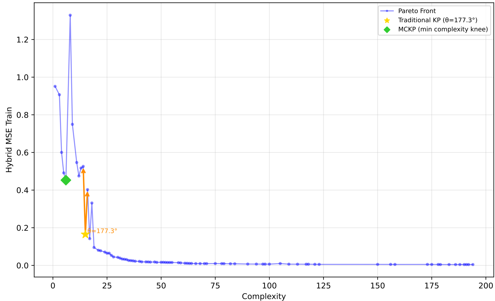
227_cpu_small - Run 18 - SVP - Hybrid MSE Train \lambda_1=0.00, \lambda_2=1.00, \lambda_3=0.00 | Difficulty: 1.00 | Method: hmr
