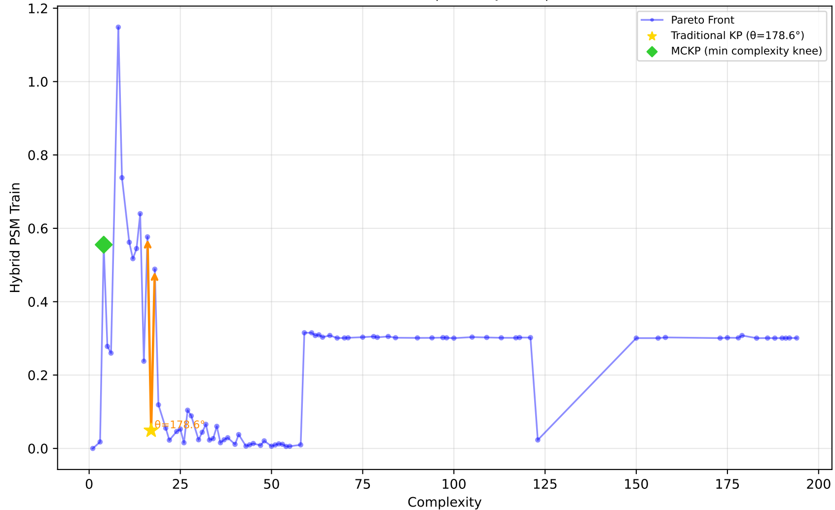
227_cpu_small - Run 18 - SVP - Hybrid PSM Train \lambda_1=0.00, \lambda_2=0.80, \lambda_3=0.30 | Difficulty: 1.00 | Method: hmr
