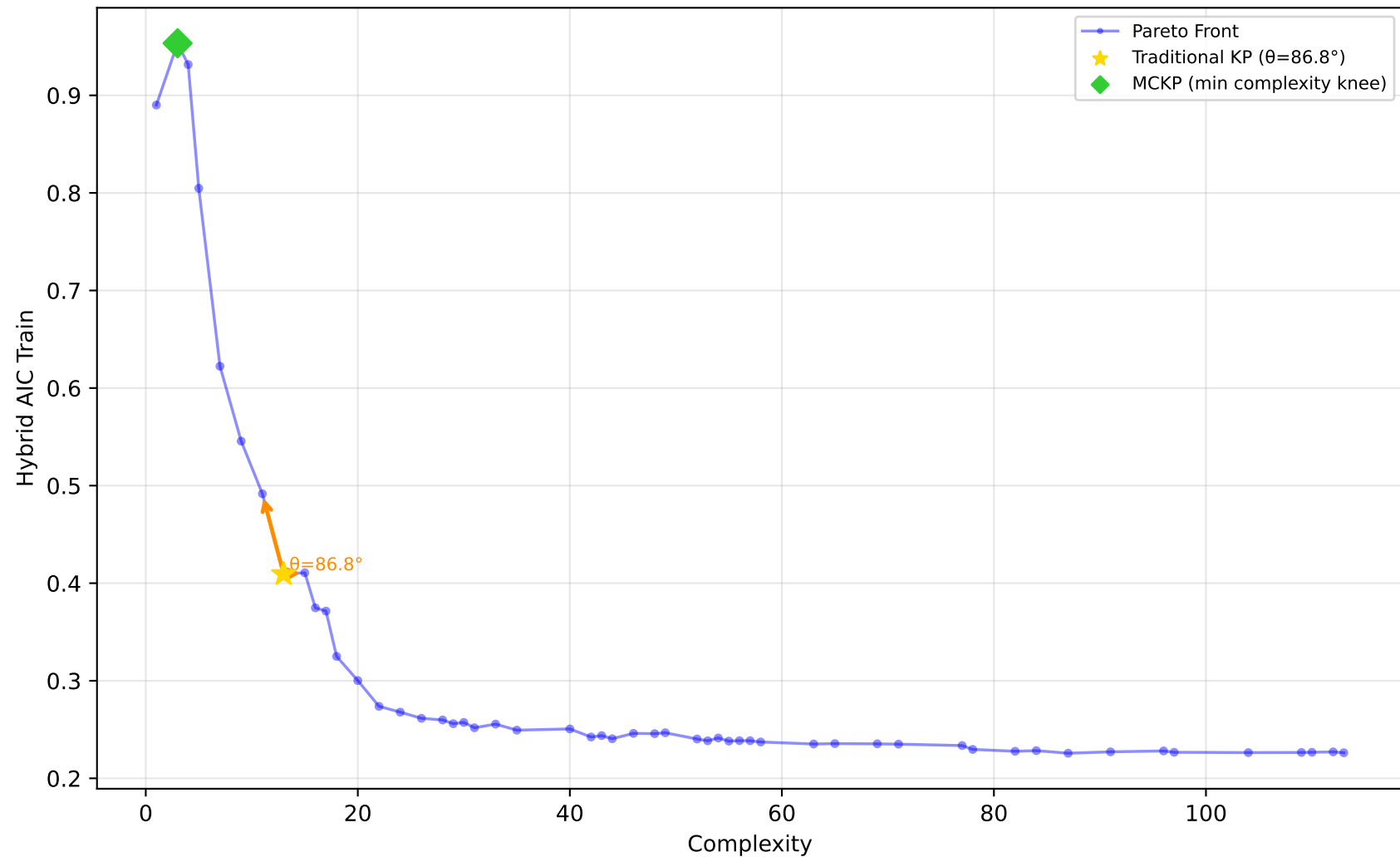
227_cpu_small - Run 19 - MVP - Hybrid AIC Train \lambda_1=0.80, \bar{\lambda}_2=0.20, \lambda_3=0.00 | Difficulty: 1.00 | Method: hmr
