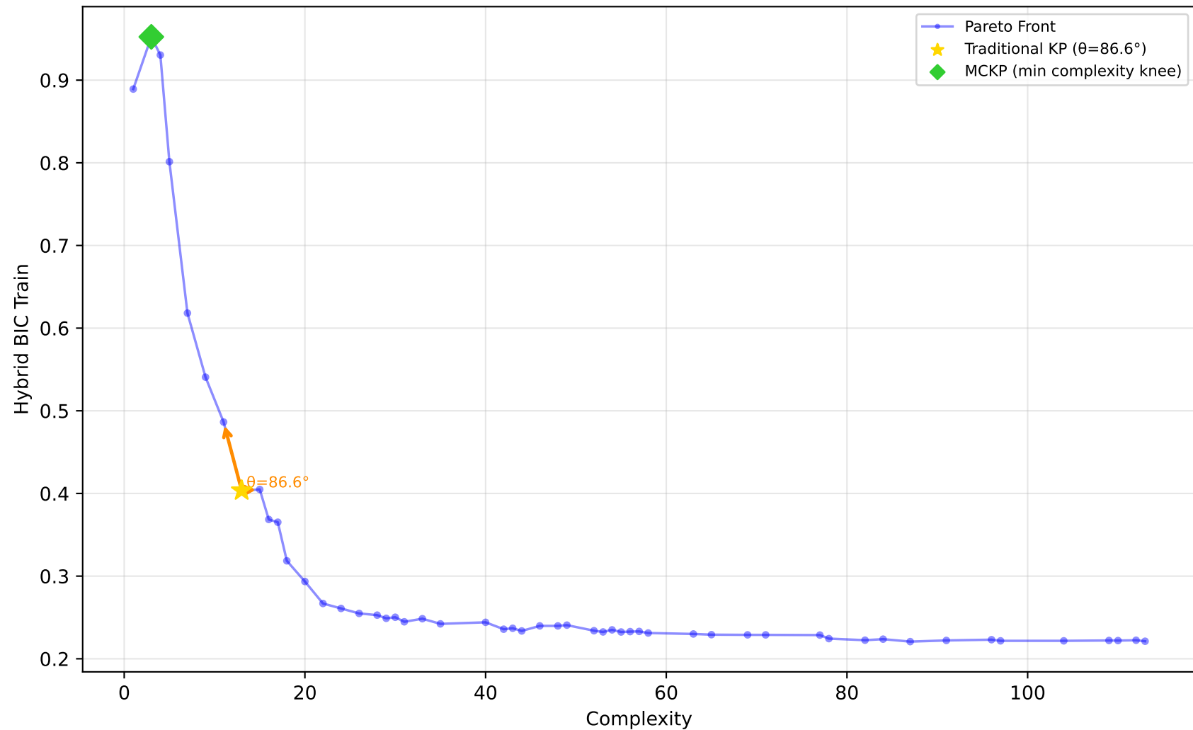
227_cpu_small - Run 19 - MVP - Hybrid BIC Train \lambda_1=0.80, \bar{\lambda}_2=0.20, \lambda_3=0.00 | Difficulty: 1.00 | Method: hmr
