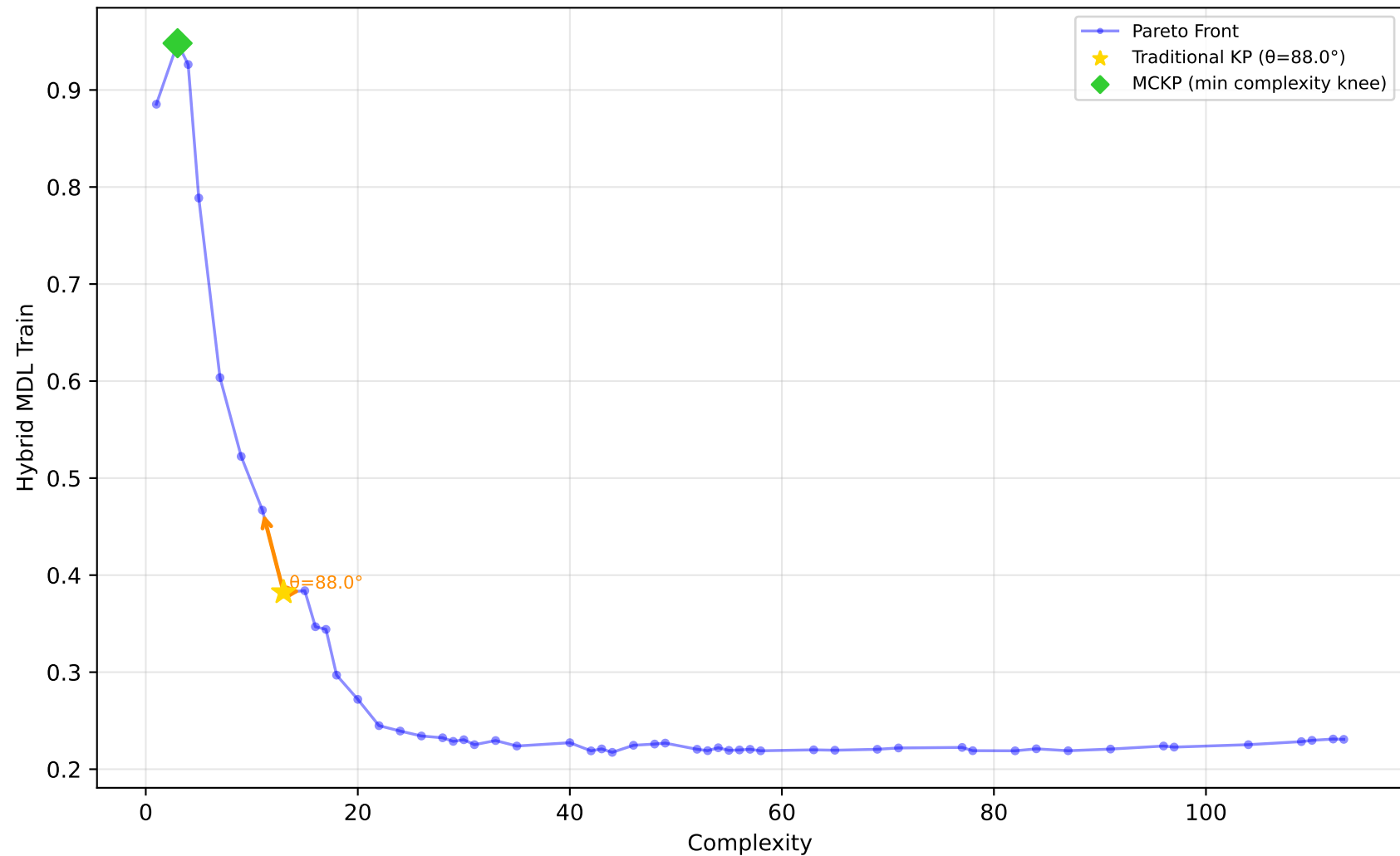
227_cpu_small - Run 19 - MVP - Hybrid MDL Train \lambda_1=0.80, \lambda_2=0.20, \lambda_3=0.00 | Difficulty: 1.00 | Method: hmr
