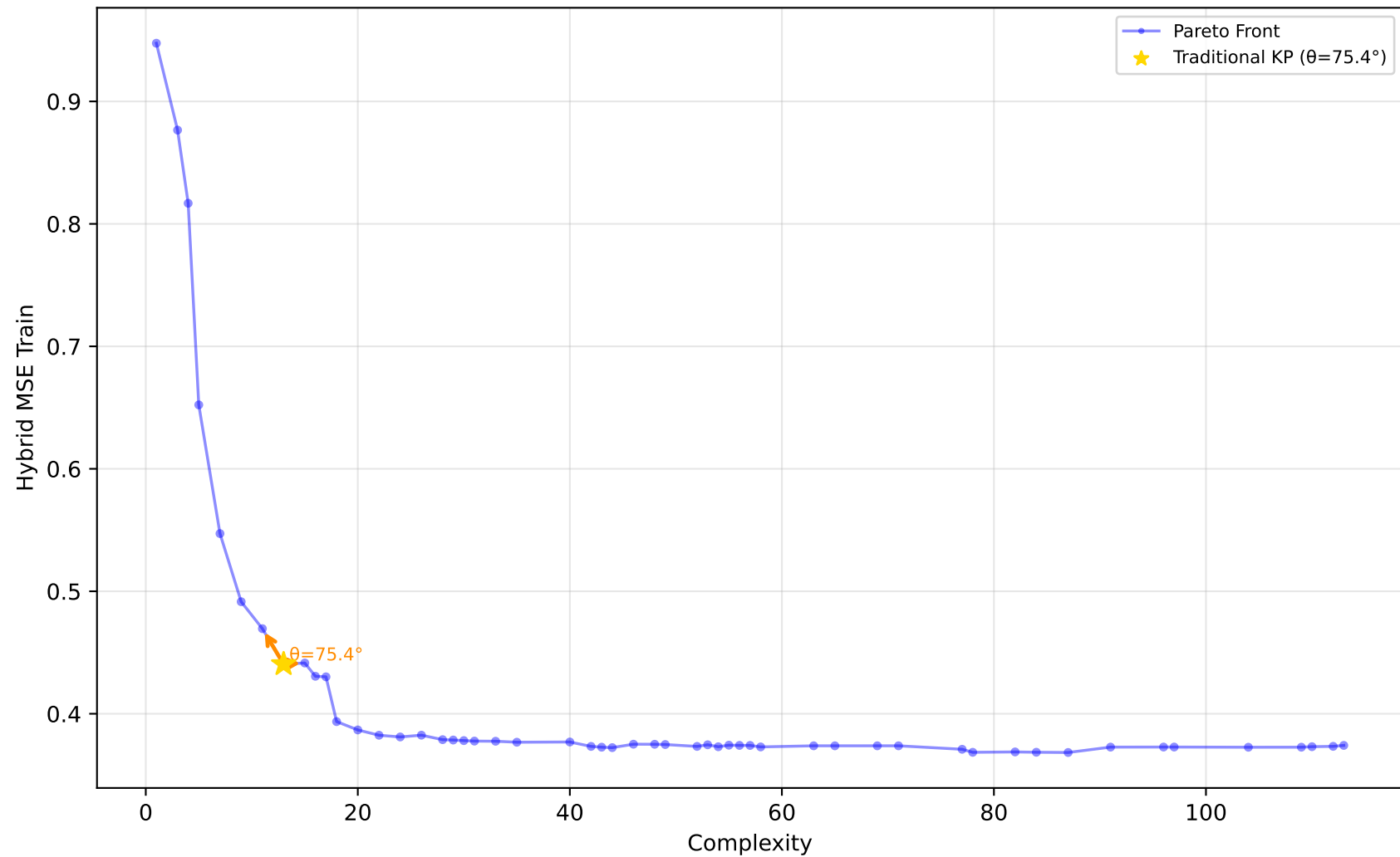
227_cpu_small - Run 19 - MVP - Hybrid MSE Train \lambda_1=0.00, \lambda_2=0.90, \lambda_3=0.10 | Difficulty: 1.00 | Method: hmr
