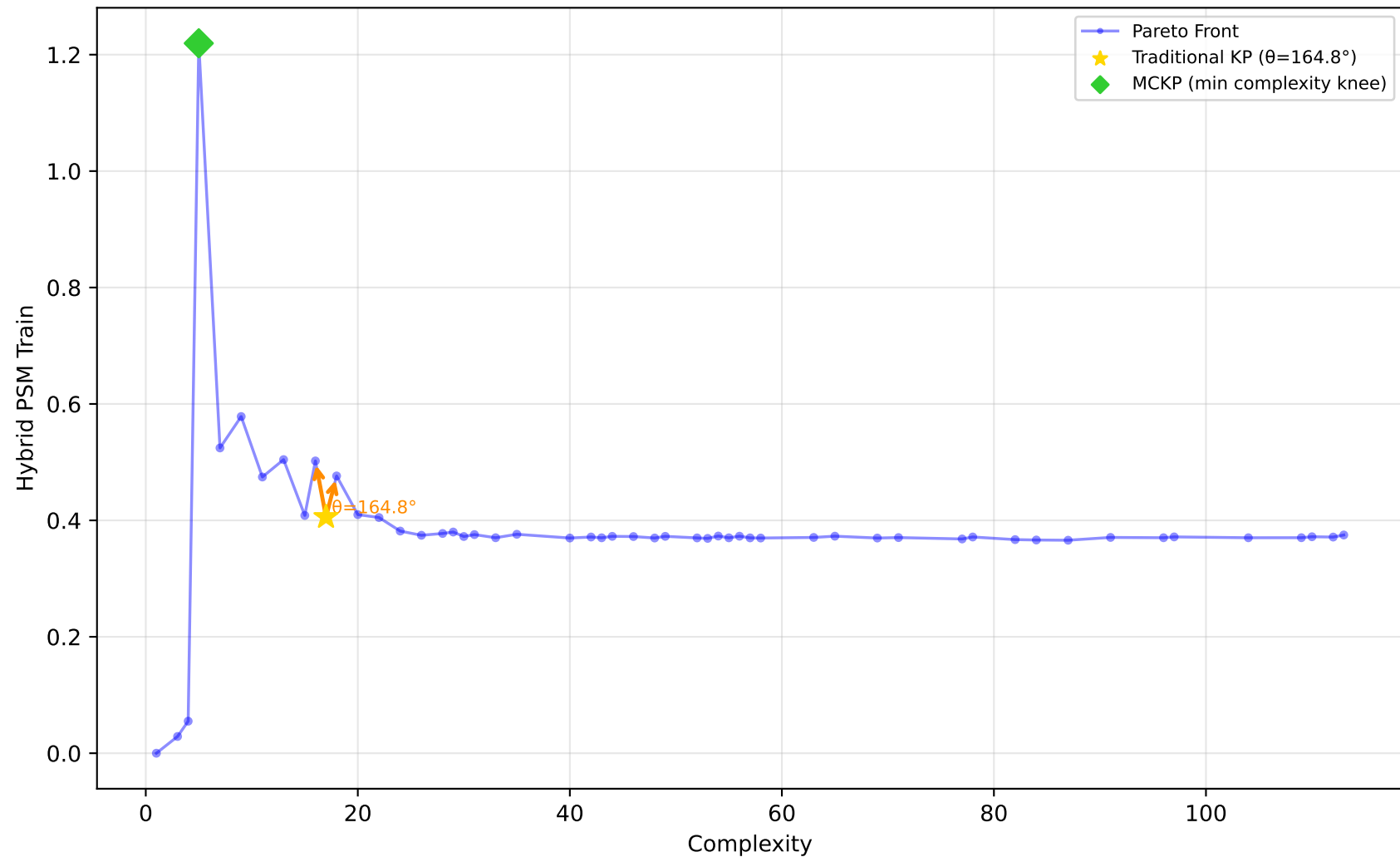
227_cpu_small - Run 19 - MVP - Hybrid PSM Train \lambda_1=0.00, \lambda_2=0.90, \lambda_3=0.10 | Difficulty: 1.00 | Method: hmr
